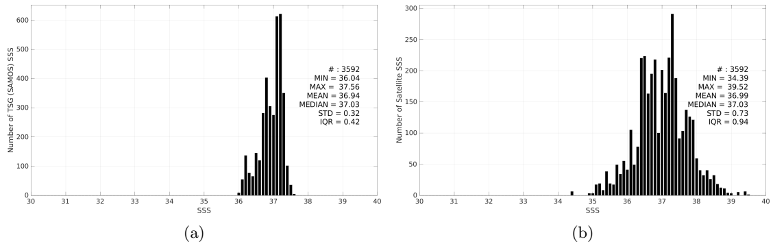
Figure 3: Histograms of SSS from TSG (SAMOS) (a) and SMAP SSS L2 v6 - 40 km (RSS) (b) considering all match-up pairs per bins of 0.1 over the SPURS 1 Pi-MEP region and for the full satellite product period.
