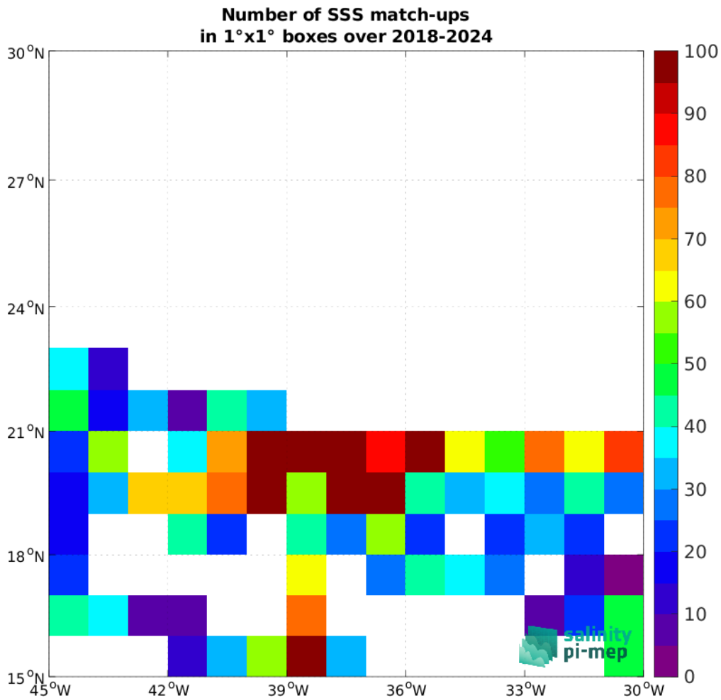
Figure 5: Number of SSS match-ups between TSG (SAMOS) SSS and the SMAP SSS L2 v6 - 40 km (RSS) SSS product for the SPURS 1 Pi-MEP region over 1°x1° boxes and for the full satellite product period.
