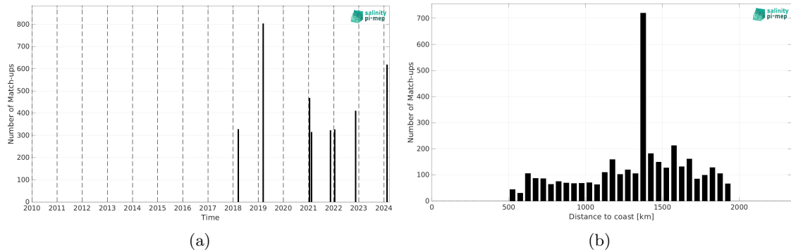
Figure 2: Number of match-ups between TSG (SAMOS) and SMAP SSS L2 v6 - 40 km (RSS) SSS as a function of time (a) and as function of the distance to coast (b) over the SPURS 1 Pi-MEP region and for the full satellite product period.
