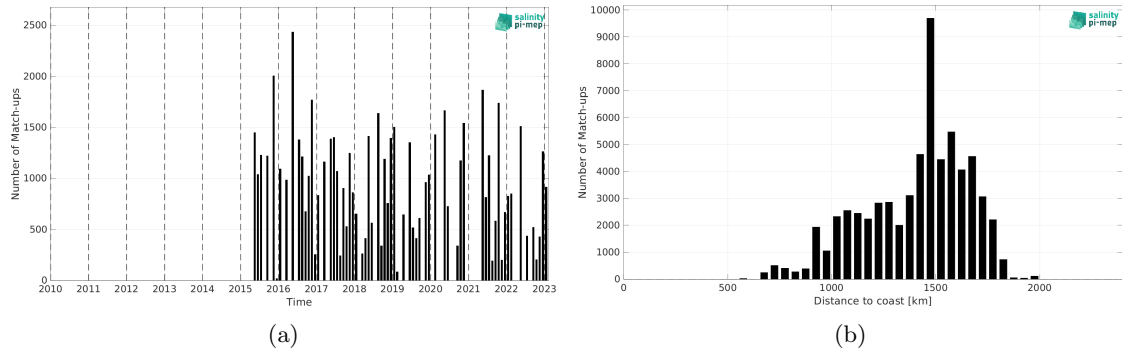
Figure 2: Number of match-ups between TSG (LEGOS-DM) and SMAP SSS L2 v6 - 40 km (RSS) SSS as a function of time (a) and as function of the distance to coast (b) over the SPURS 1 Pi-MEP region and for the full satellite product period.
