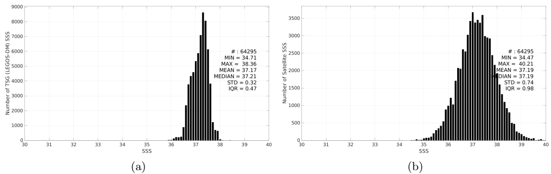
Figure 3: Histograms of SSS from TSG (LEGOS-DM) (a) and SMAP SSS L2 v6 - 40 km (RSS) (b) considering all match-up pairs per bins of 0.1 over the SPURS 1 Pi-MEP region and for the full satellite product period.
