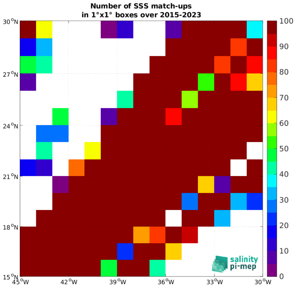
Figure 5: Number of SSS match-ups between TSG (LEGOS-DM) SSS and the SMAP SSS L2 v6 - 40 km (RSS) SSS product for the SPURS 1 Pi-MEP region over 1^\circ \times 1^\circ boxes and for the full satellite product period.
