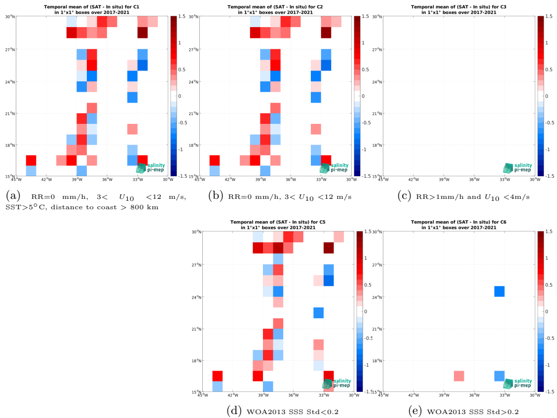
Figure 14: Temporal mean gridded over spatial boxes of size 1^\circ \times 1^\circ of \Delta SSS (SMAP SSS L2 v6 - 40 km (RSS) - TSG (GOSUD-Sailing-ship)) for 5 different subdatasets corresponding to: RR=0 mm/h, 3 < U_{10} < 12 m/s, SST > 5^\circ C , distance to coast > 800 km (a), RR=0 mm/h, 3 < U_{10} < 12 m/s (b), RR > 1 mm/h and U_{10} < 4 m/s (c), WOA2013 SSS Std <0.2 (d), WOA2013 SSS Std >0.2 (e).
