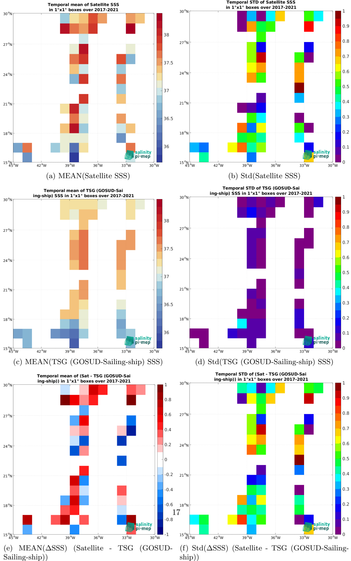
Figure 7: Temporal mean (left) and Std (right) of SSS from SMAP SSS L2 v6 - 40 km (RSS) (top), TSG (GOSUD-Sailing-ship) (middle), and of \Delta SSS (Satellite - TSG (GOSUD-Sailing-ship)). Only match-up pairs are used to generate these maps.
