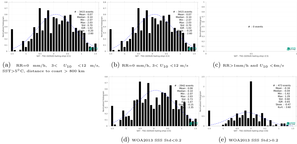
Figure 15: Normalized histogram of \Delta SSS (SMAP SSS L2 v6 - 40 km (RSS) - TSG (GOSUD-Sailing-ship)) for 5 different subdatasets corresponding to: RR=0 mm/h, 3 < U_{10} < 12 m/s, SST > 5°C, distance to coast > 800 km (a), RR=0 mm/h, 3 < U_{10} < 12 m/s (b), RR > 1mm/h and U_{10} < 4 m/s (c), WOA2013 SSS Std < 0.2 (d), WOA2013 SSS Std > 0.2 (e).
