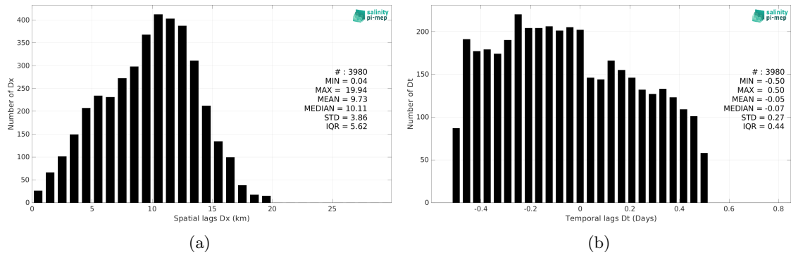
Figure 6: Histograms of the spatial (a) and temporal (b) lags between the location/time of the TSG (GOSUD-Sailing-ship) measurement and the date of the corresponding SMAP SSS L2 v6 - 40 km (RSS) SSS pixel.
