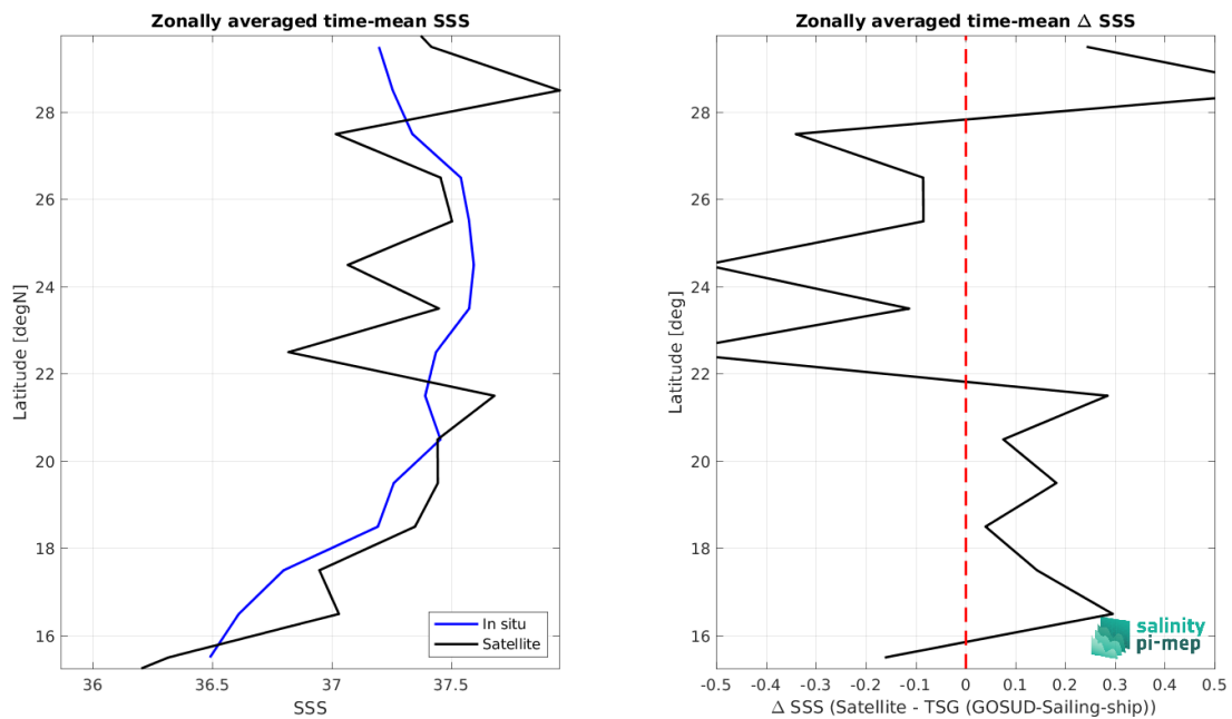
Figure 9: Left panel: Zonal mean SSS from SMAP SSS L2 v6 - 40 km (RSS) satellite product (black) and from TSG (GOSUD-Sailing-ship) (blue). Right panel: Zonal mean of \Delta SSS (Satellite - TSG (GOSUD-Sailing-ship)) for all the collected Pi-MEP match-up pairs estimated over the full satellite product period.
