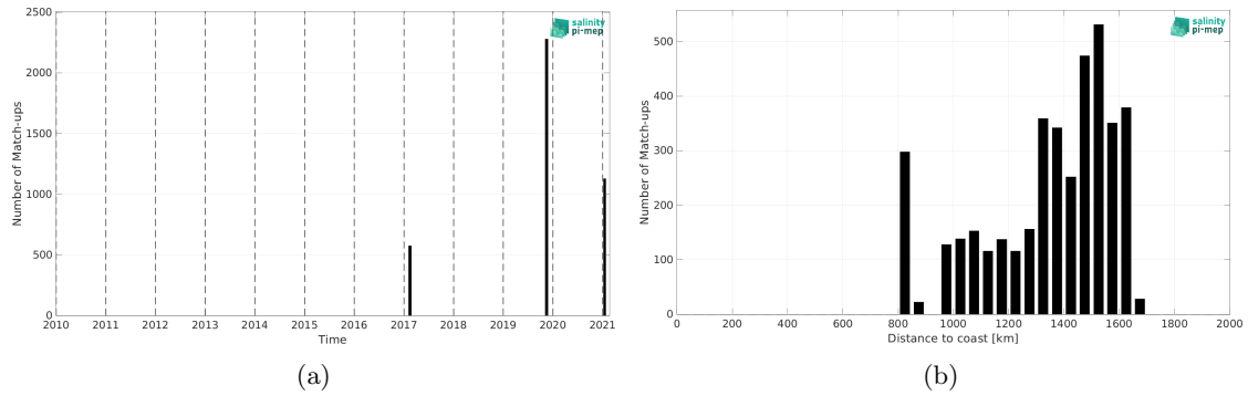
Figure 2: Number of match-ups between TSG (GOSUD-Sailing-ship) and SMAP SSS L2 v6 - 40 km (RSS) SSS as a function of time (a) and as function of the distance to coast (b) over the SPURS 1 Pi-MEP region and for the full satellite product period.
