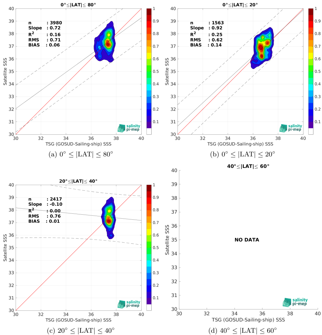
Figure 10: Contour maps of the concentration of SMAP SSS L2 v6 - 40 km (RSS) SSS (y-axis) versus TSG (GOSUD-Sailing-ship) SSS (x-axis) at match-up pairs for different latitude bands. For each plot, the red line shows x=y . The black thin and dashed lines indicate a linear fit through the data cloud and the \pm 95\% confidence levels, respectively. The number match-up pairs n , the slope and R^2 coefficient of the linear fit, the root mean square (RMS) and the mean bias between satellite and in situ data are indicated for each latitude band in each plots.
