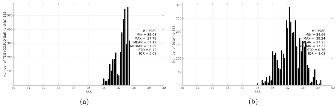
Figure 3: Histograms of SSS from TSG (GOSUD-Sailing-ship) (a) and SMAP SSS L2 v6 - 40 km (RSS) (b) considering all match-up pairs per bins of 0.1 over the SPURS 1 Pi-MEP region and for the full satellite product period.
