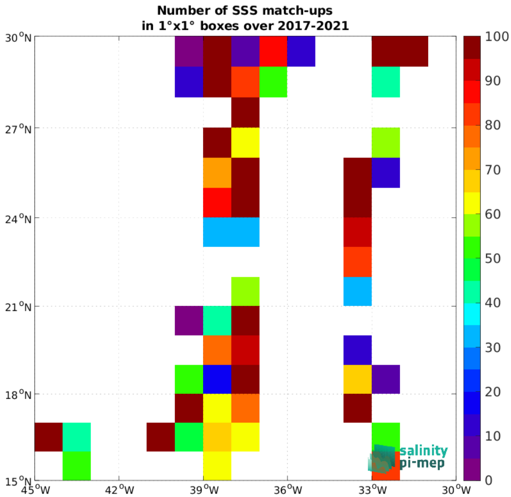
Figure 5: Number of SSS match-ups between TSG (GOSUD-Sailing-ship) SSS and the SMAP SSS L2 v6 - 40 km (RSS) SSS product for the SPURS 1 Pi-MEP region over 1°x1° boxes and for the full satellite product period.
