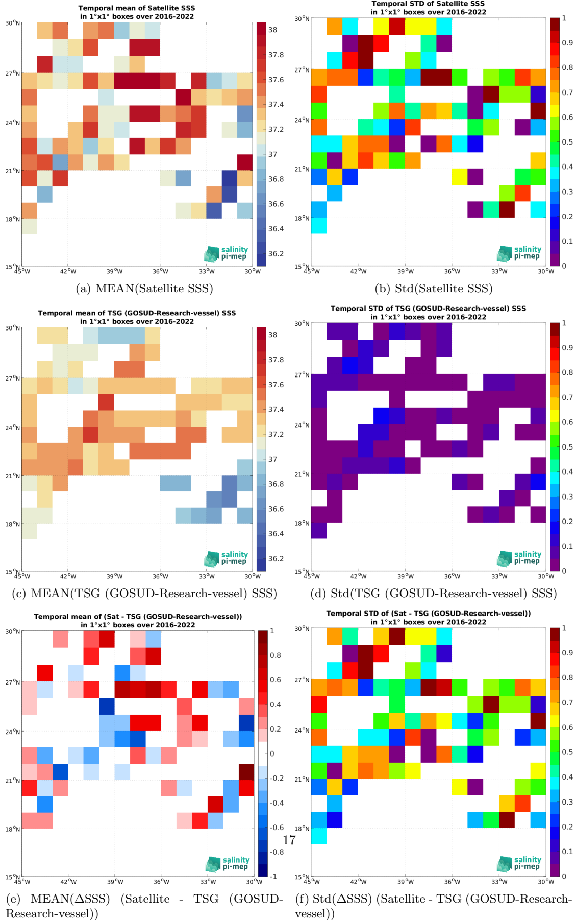
Figure 7: Temporal mean (left) and Std (right) of SSS from SMAP SSS L2 v6 - 40 km (RSS) (top), TSG (GOSUD-Research-vessel) (middle), and of \Delta SSS (Satellite - TSG (GOSUD-Research-vessel)). Only match-up pairs are used to generate these maps.
