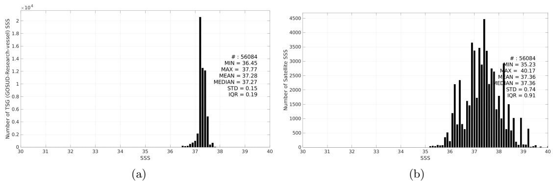
Figure 3: Histograms of SSS from TSG (GOSUD-Research-vessel) (a) and SMAP SSS L2 v6 - 40 km (RSS) (b) considering all match-up pairs per bins of 0.1 over the SPURS 1 Pi-MEP region and for the full satellite product period.
