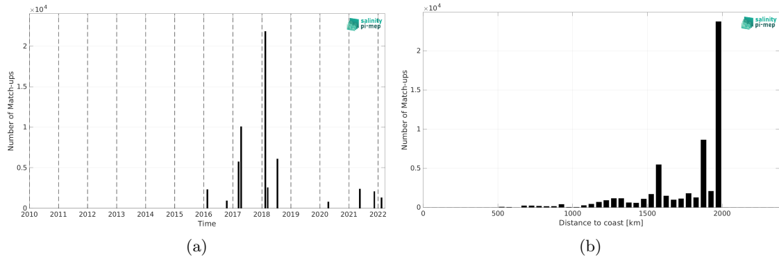
Figure 2: Number of match-ups between TSG (GOSUD-Research-vessel) and SMAP SSS L2 v6 - 40 km (RSS) SSS as a function of time (a) and as function of the distance to coast (b) over the SPURS 1 Pi-MEP region and for the full satellite product period.
