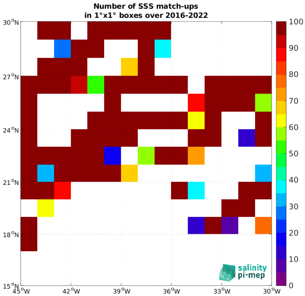
Figure 5: Number of SSS match-ups between TSG (GOSUD-Research-vessel) SSS and the SMAP SSS L2 v6 - 40 km (RSS) SSS product for the SPURS 1 Pi-MEP region over 1°x1° boxes and for the full satellite product period.
