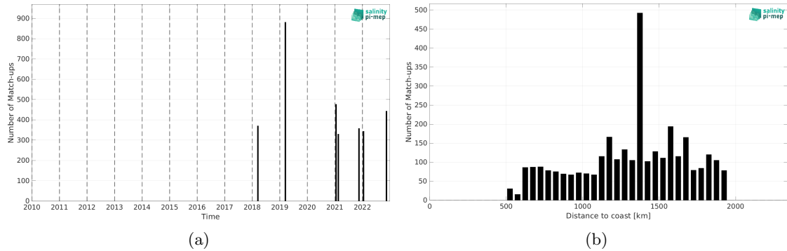
Figure 1: Number of match-ups between TSG (SAMOS) and SMAP SSS L2 v5 (RSS) SSS as a function of time (a) and as function of the distance to coast (b) over the SPURS 1 Pi-MEP region and for the full satellite product period.
