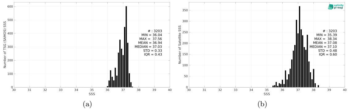
Figure 2: Histograms of SSS from TSG (SAMOS) (a) and SMAP SSS L2 v5 (RSS) (b) considering all match-up pairs per bins of 0.1 over the SPURS 1 Pi-MEP region and for the full satellite product period.
