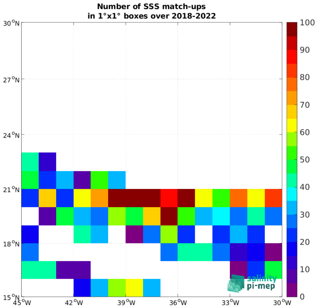
Figure 4: Number of SSS match-ups between TSG (SAMOS) SSS and the SMAP SSS L2 v5 (RSS) SSS product for the SPURS 1 Pi-MEP region over 1°x1° boxes and for the full satellite product period.
