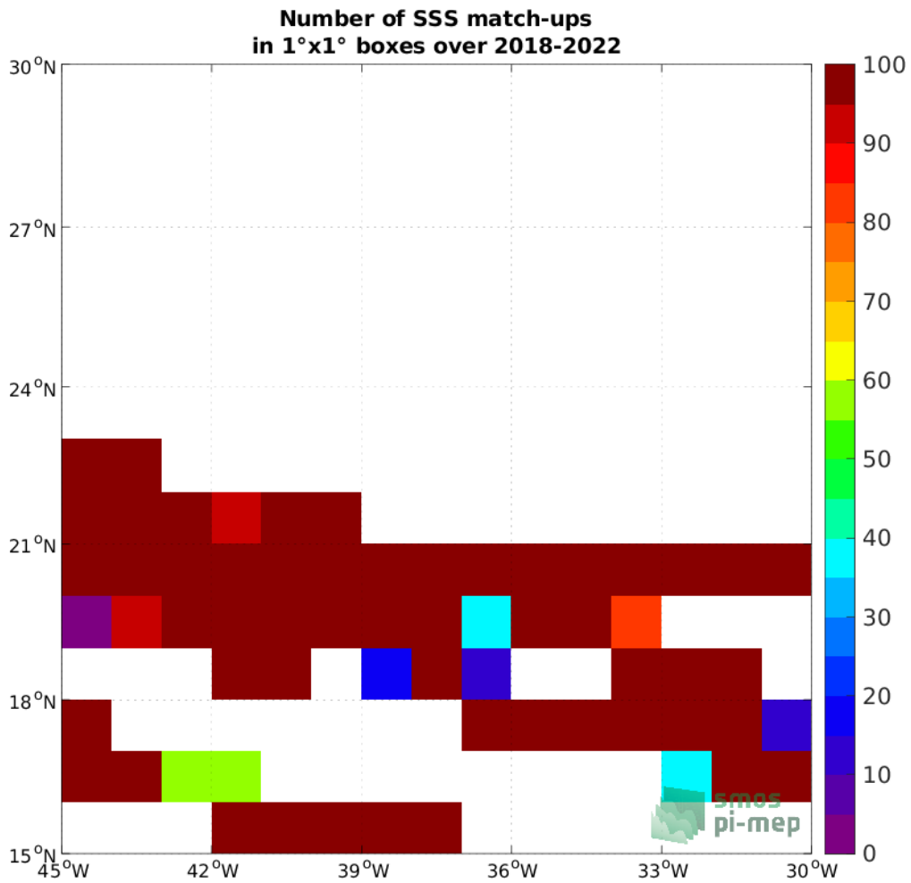
Figure 4: Number of SSS match-ups between TSG (SAMOS) SSS and the SMAP SSS L2 v5 (RSS) SSS product for the SPURS 1 Pi-MEP region over 1^\circ \times 1^\circ boxes and for the full satellite product period.
