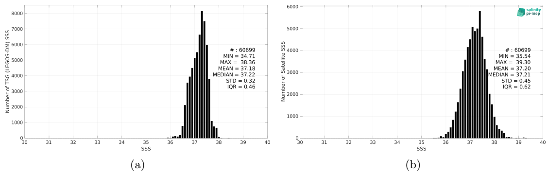
Figure 2: Histograms of SSS from TSG (LEGOS-DM) (a) and SMAP SSS L2 v5 (RSS) (b) considering all match-up pairs per bins of 0.1 over the SPURS 1 Pi-MEP region and for the full satellite product period.
