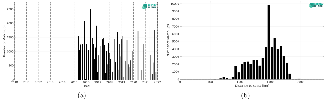
Figure 1: Number of match-ups between TSG (LEGOS-DM) and SMAP SSS L2 v5 (RSS) SSS as a function of time (a) and as function of the distance to coast (b) over the SPURS 1 Pi-MEP region and for the full satellite product period.
