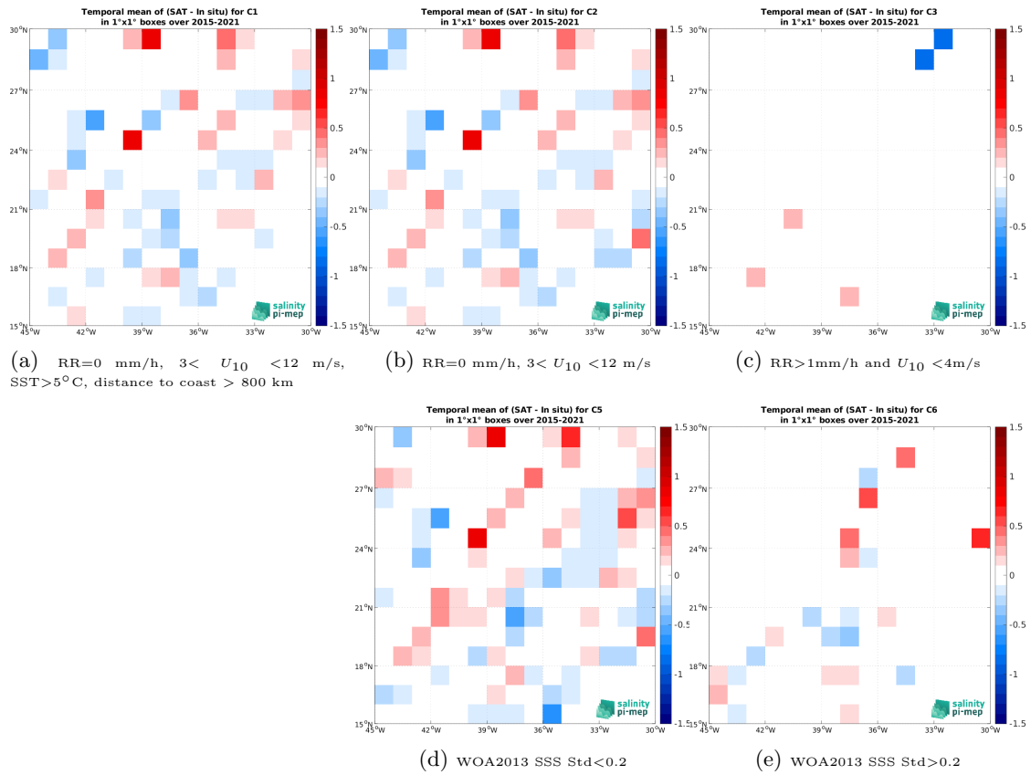
Figure 12: Temporal mean gridded over spatial boxes of size 1^\circ \times 1^\circ of \Delta SSS (SMAP SSS L2 v5 (RSS) - TSG (LEGOS-DM)) for 5 different subdatasets corresponding to:RR=0 mm/h, 3 < U_{10} < 12 m/s, SST >5^\circ\text{C} , distance to coast > 800 km (a), RR=0 mm/h, 3 < U_{10} < 12 m/s (b), RR >1 mm/h and U_{10} < 4 m/s (c), WOA2013 SSS Std <0.2 (d), WOA2013 SSS Std >0.2 (e).
