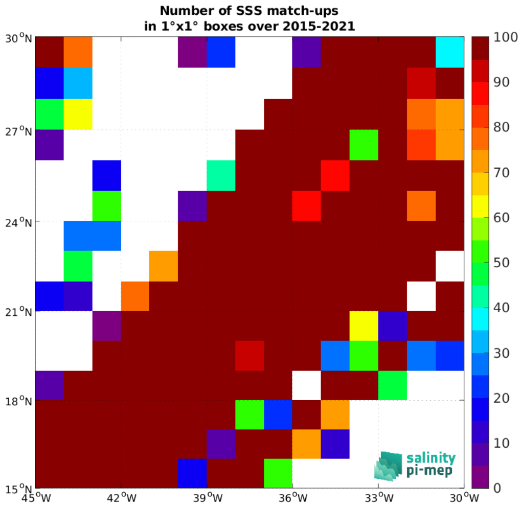
Figure 4: Number of SSS match-ups between TSG (LEGOS-DM) SSS and the SMAP SSS L2 v5 (RSS) SSS product for the SPURS 1 Pi-MEP region over 1^\circ \times 1^\circ boxes and for the full satellite product period.
