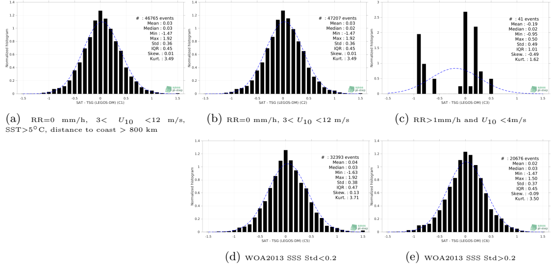
Figure 13: Normalized histogram of \Delta SSS (SMAP SSS L2 v5 (RSS) - TSG (LEGOS-DM)) for 5 different subdatasets corresponding to: RR=0 mm/h, 3 < U_{10} < 12 m/s, SST>5°C, distance to coast > 800 km (a), RR=0 mm/h, 3 < U_{10} < 12 m/s (b), RR>1mm/h and U_{10} < 4 m/s (c), WOA2013 SSS Std<0.2 (d), WOA2013 SSS Std>0.2 (e).
