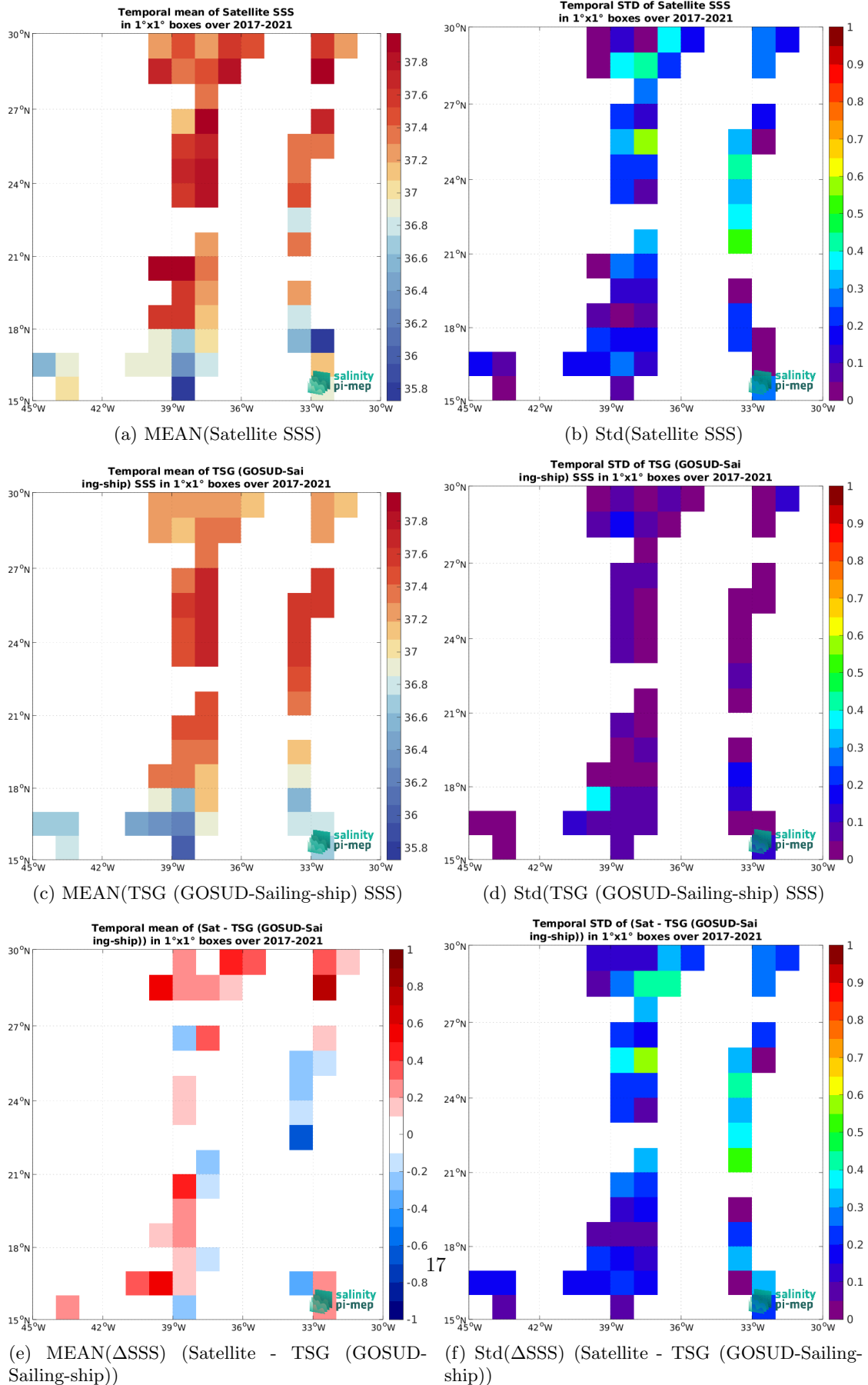
Figure 6: Temporal mean (left) and Std (right) of SSS from SMAP SSS L2 v5 (RSS) (top), TSG (GOSUD-Sailing-ship) (middle), and of \Delta SSS (Satellite - TSG (GOSUD-Sailing-ship)). Only match-up pairs are used to generate these maps.
