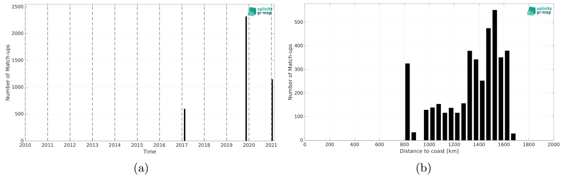
Figure 1: Number of match-ups between TSG (GOSUD-Sailing-ship) and SMAP SSS L2 v5 (RSS) SSS as a function of time (a) and as function of the distance to coast (b) over the SPURS 1 Pi-MEP region and for the full satellite product period.
