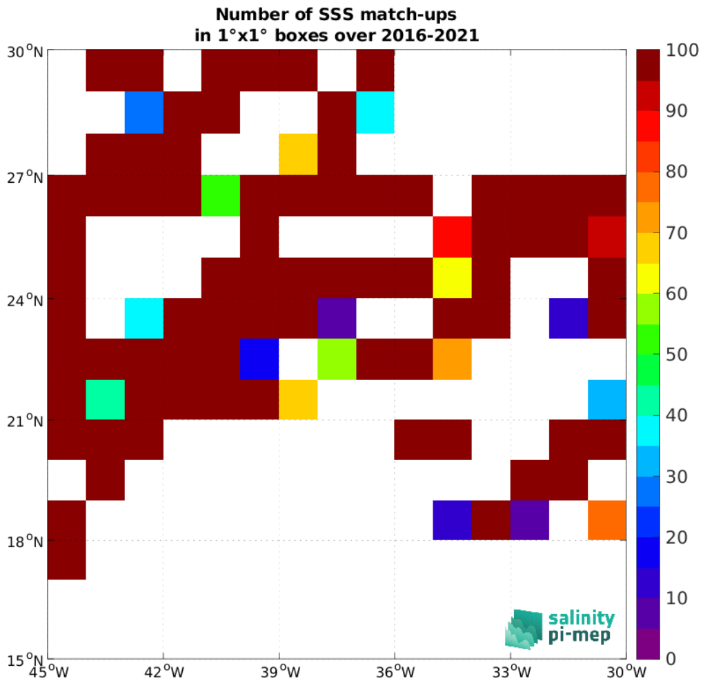
Figure 4: Number of SSS match-ups between TSG (GOSUD-Research-vessel) SSS and the SMAP SSS L2 v5 (RSS) SSS product for the SPURS 1 Pi-MEP region over 1^\circ \times 1^\circ boxes and for the full satellite product period.
