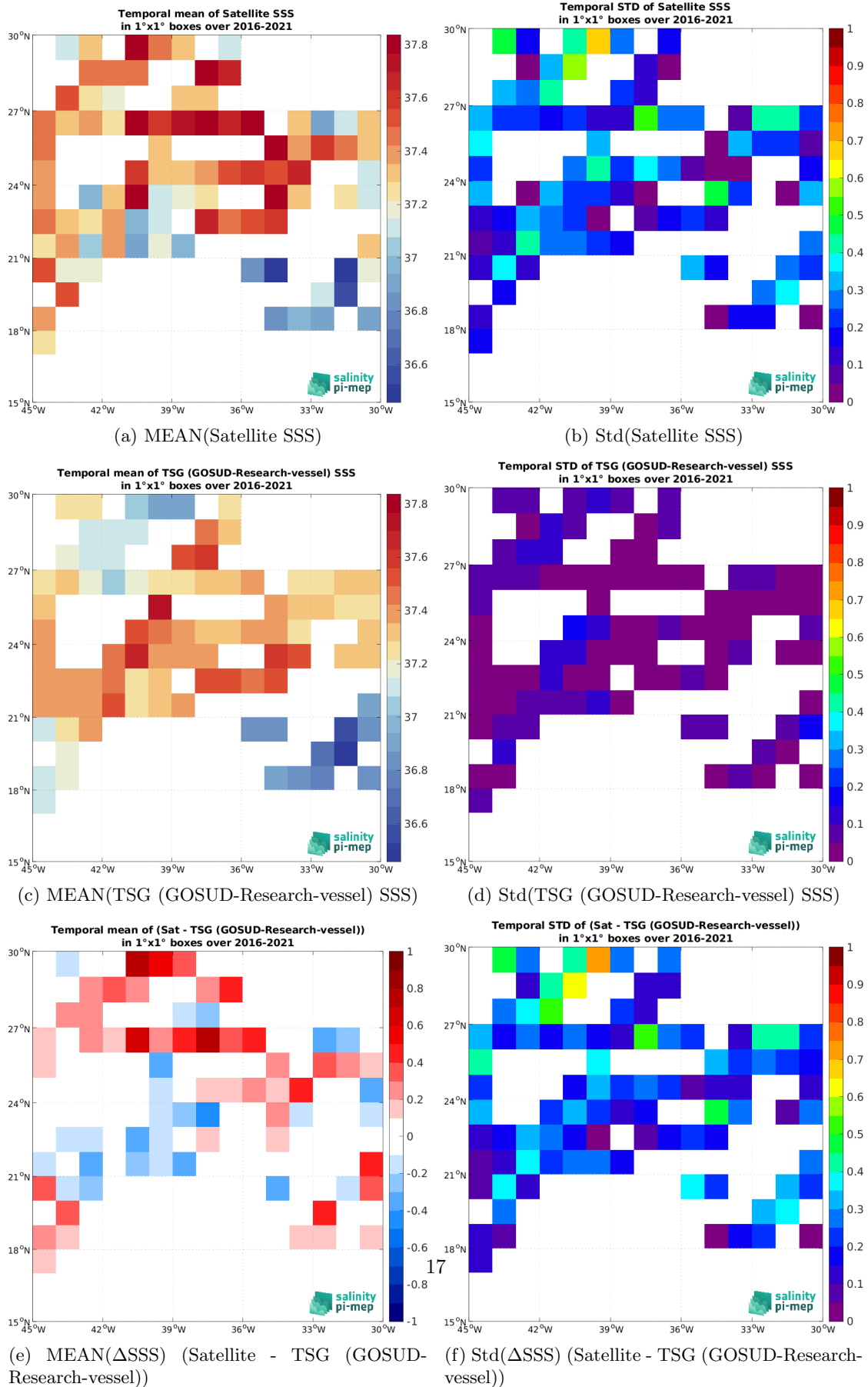
Figure 6: Temporal mean (left) and Std (right) of SSS from SMAP SSS L2 v5 (RSS) (top), TSG (GOSUD-Research-vessel) (middle), and of \Delta SSS (Satellite - TSG (GOSUD-Research-vessel)). Only match-up pairs are used to generate these maps.
