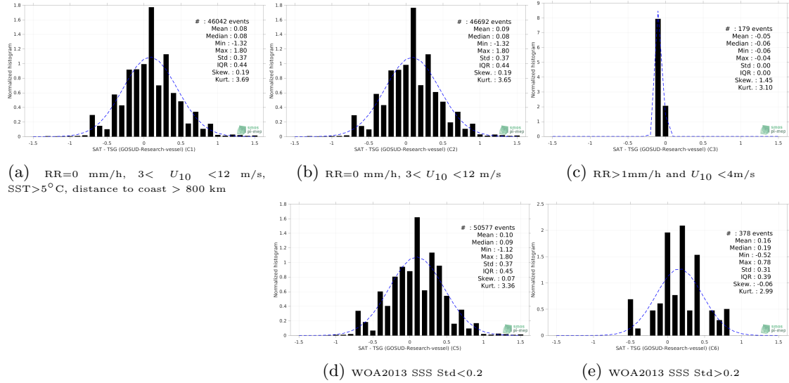
Figure 13: Normalized histogram of \Delta\text{SSS} (SMAP SSS L2 v5 (RSS) - TSG (GOSUD-Research-vessel)) for 5 different subdatasets corresponding to: RR=0 mm/h, 3 < U_{10} < 12 m/s, SST > 5^{\circ}\text{C} , distance to coast > 800 km (a), RR=0 mm/h, 3 < U_{10} < 12 m/s (b), RR > 1\text{mm/h} and U_{10} < 4\text{m/s} (c), WOA2013 SSS Std < 0.2 (d), WOA2013 SSS Std > 0.2 (e).
