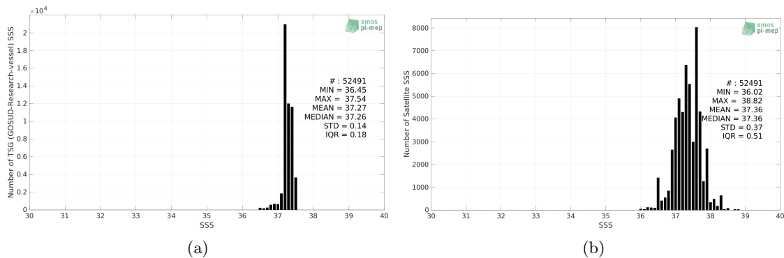
Figure 2: Histograms of SSS from TSG (GOSUD-Research-vessel) (a) and SMAP SSS L2 v5 (RSS) (b) considering all match-up pairs per bins of 0.1 over the SPURS 1 Pi-MEP region and for the full satellite product period.
