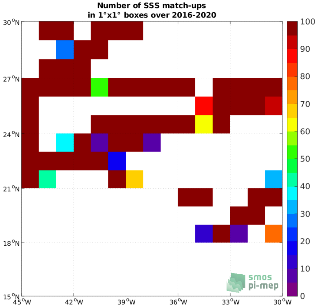
Figure 4: Number of SSS match-ups between TSG (GOSUD-Research-vessel) SSS and the SMAP SSS L2 v5 (RSS) SSS product for the SPURS 1 Pi-MEP region over 1°x1° boxes and for the full satellite product period.
