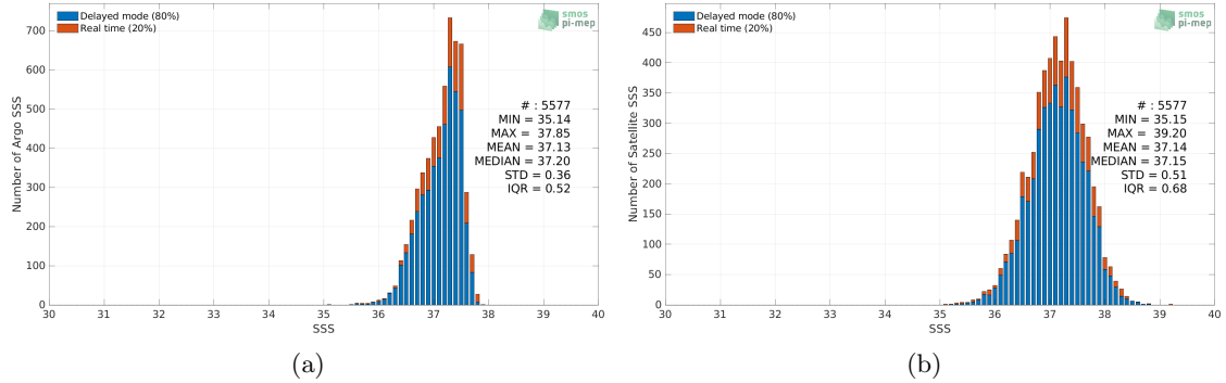
Figure 2: Histograms of SSS from Argo (a) and SMAP SSS L2 v5 (RSS) (b) considering all match-up pairs per bins of 0.1 over the SPURS 1 Pi-MEP region and for the full satellite product period.
