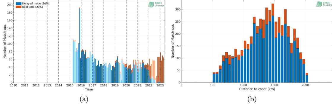
Figure 1: Number of match-ups between Argo and SMAP SSS L2 v5 (RSS) SSS as a function of time (a) and as function of the distance to coast (b) over the SPURS 1 Pi-MEP region and for the full satellite product period.
