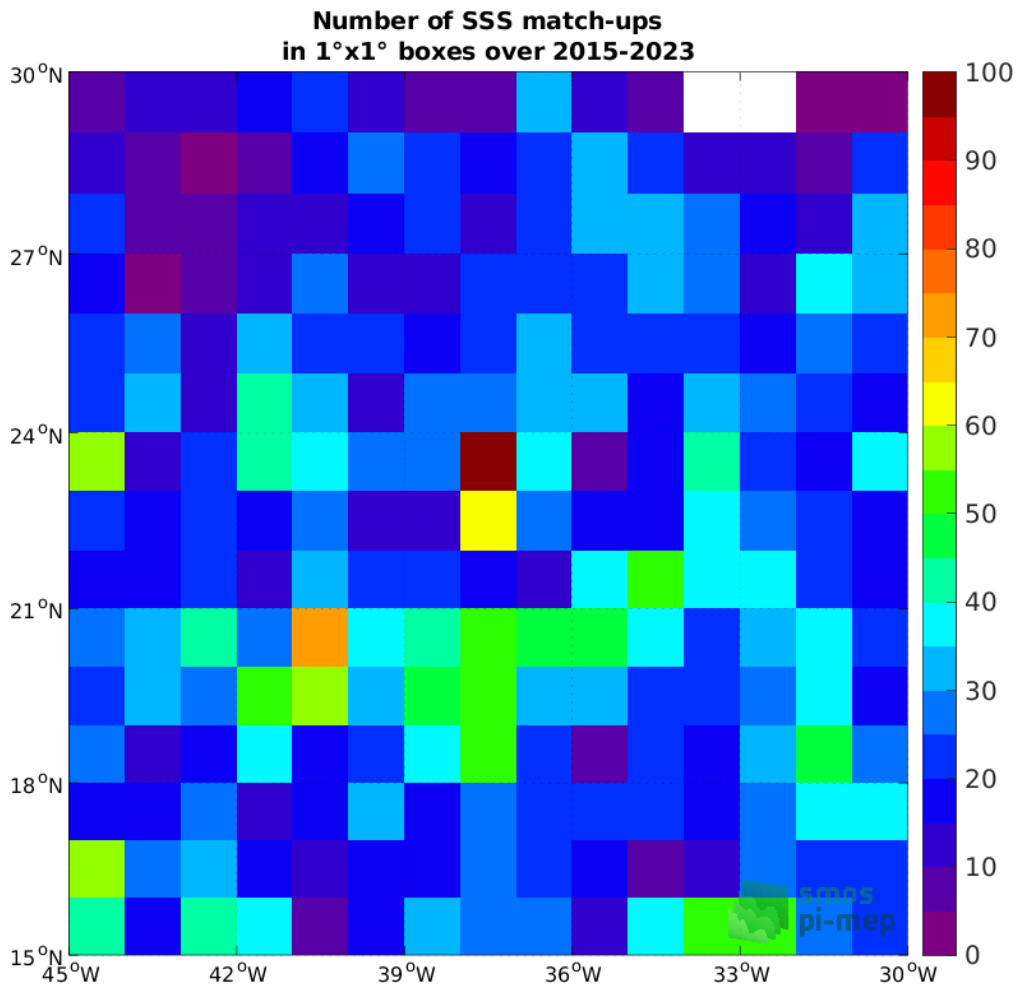
Figure 4: Number of SSS match-ups between Argo SSS and the SMAP SSS L2 v5 (RSS) SSS product for the SPURS 1 Pi-MEP region over 1°×1° boxes and for the full satellite product period.
