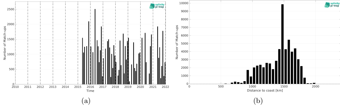
Figure 2: Number of match-ups between TSG (LEGOS-DM) and SMAP SSS L2 v5.3 (RSS) SSS as a function of time (a) and as function of the distance to coast (b) over the SPURS 1 Pi-MEP region and for the full satellite product period.
