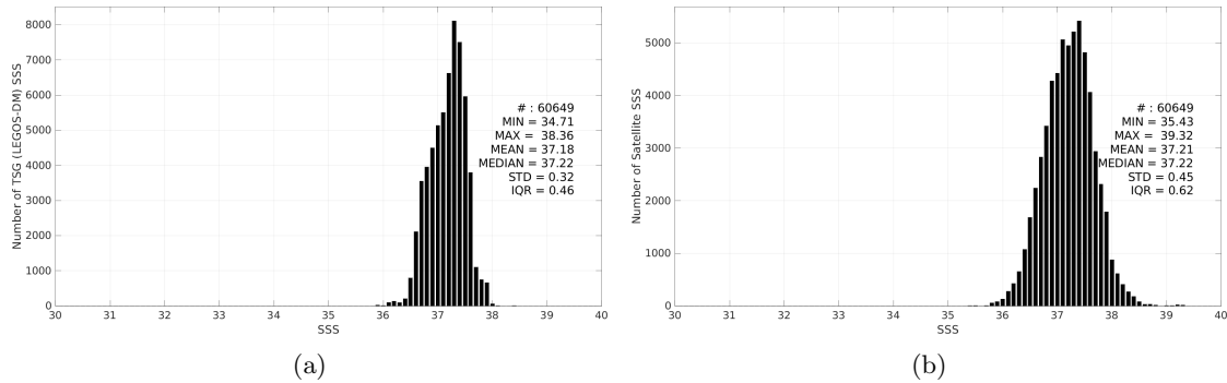
Figure 3: Histograms of SSS from TSG (LEGOS-DM) (a) and SMAP SSS L2 v5.3 (RSS) (b) considering all match-up pairs per bins of 0.1 over the SPURS 1 Pi-MEP region and for the full satellite product period.
