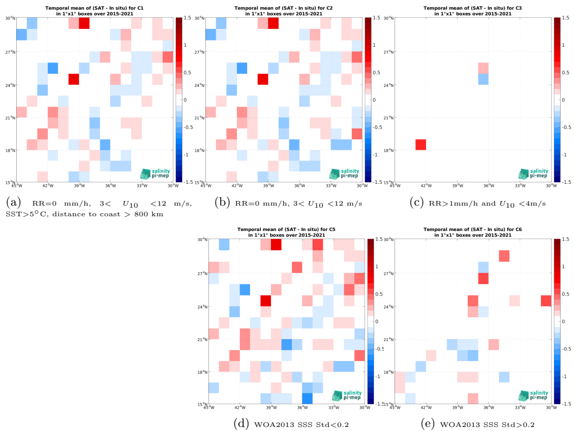
Figure 14: Temporal mean gridded over spatial boxes of size 1^\circ \times 1^\circ of \Delta SSS (SMAP SSS L2 v5.3 (RSS) - TSG (LEGOS-DM)) for 5 different subdatasets corresponding to: RR=0 mm/h, 3 < U_{10} < 12 m/s, SST > 5^\circ C , distance to coast > 800 km (a), RR=0 mm/h, 3 < U_{10} < 12 m/s (b), RR > 1 mm/h and U_{10} < 4 m/s (c), WOA2013 SSS Std < 0.2 (d), WOA2013 SSS Std > 0.2 (e).
