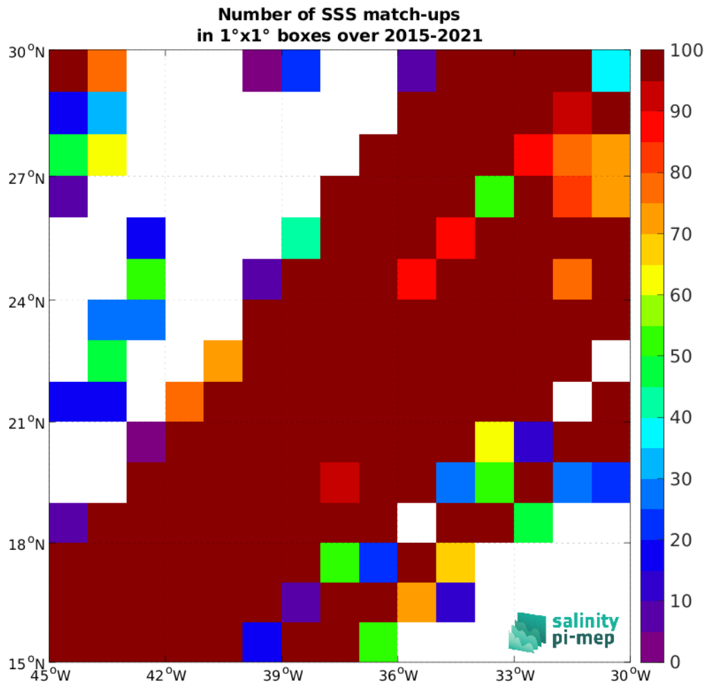
Figure 5: Number of SSS match-ups between TSG (LEGOS-DM) SSS and the SMAP SSS L2 v5.3 (RSS) SSS product for the SPURS 1 Pi-MEP region over 1^\circ \times 1^\circ boxes and for the full satellite product period.
