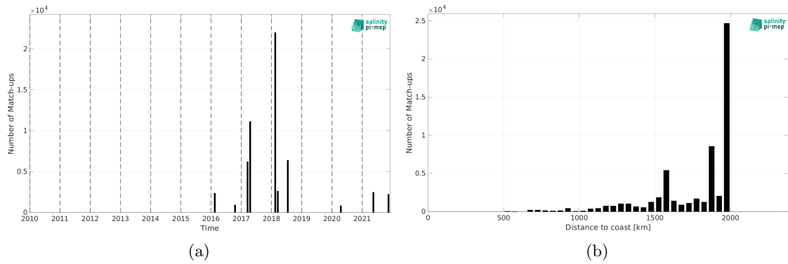
Figure 2: Number of match-ups between TSG (GOSUD-Research-vessel) and SMAP SSS L2 v5.3 (RSS) SSS as a function of time (a) and as function of the distance to coast (b) over the SPURS 1 Pi-MEP region and for the full satellite product period.
