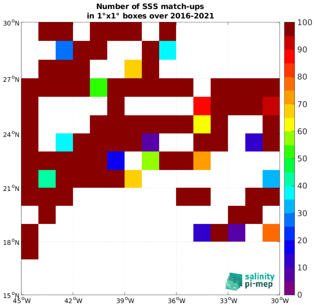
Figure 5: Number of SSS match-ups between TSG (GOSUD-Research-vessel) SSS and the SMAP SSS L2 v5.3 (RSS) SSS product for the SPURS 1 Pi-MEP region over 1^\circ \times 1^\circ boxes and for the full satellite product period.
