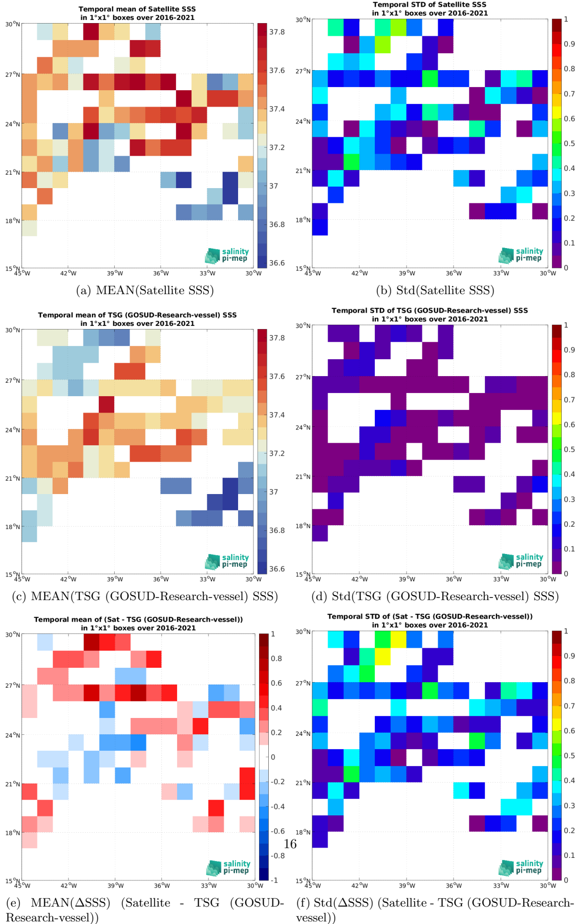
Figure 7: Temporal mean (left) and Std (right) of SSS from SMAP SSS L2 v5.3 (RSS) (top), TSG (GOSUD-Research-vessel) (middle), and of \Delta SSS (Satellite - TSG (GOSUD-Research-vessel)). Only match-up pairs are used to generate these maps.
