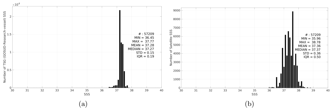
Figure 3: Histograms of SSS from TSG (GOSUD-Research-vessel) (a) and SMAP SSS L2 v5.3 (RSS) (b) considering all match-up pairs per bins of 0.1 over the SPURS 1 Pi-MEP region and for the full satellite product period.
