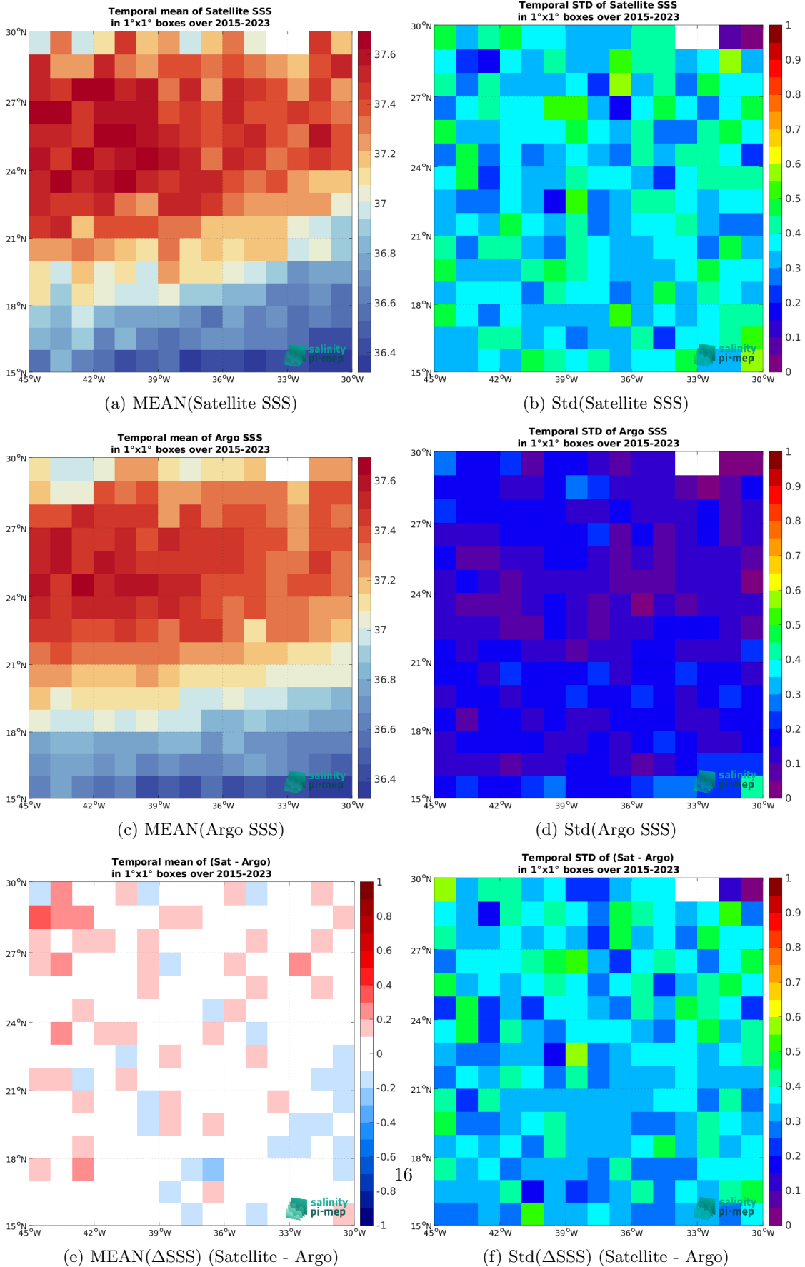
Figure 7: Temporal mean (left) and Std (right) of SSS from SMAP SSS L2 v5.3 (RSS) (top), Argo (middle), and of \Delta SSS (Satellite - Argo). Only match-up pairs are used to generate these maps.
