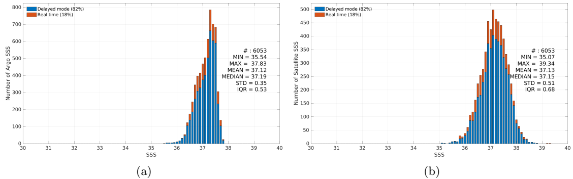
Figure 3: Histograms of SSS from Argo (a) and SMAP SSS L2 v5.3 (RSS) (b) considering all match-up pairs per bins of 0.1 over the SPURS 1 Pi-MEP region and for the full satellite product period.
