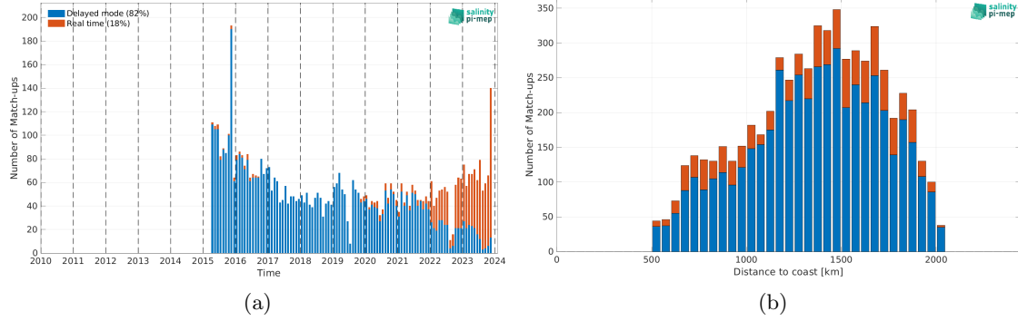
Figure 2: Number of match-ups between Argo and SMAP SSS L2 v5.3 (RSS) SSS as a function of time (a) and as function of the distance to coast (b) over the SPURS 1 Pi-MEP region and for the full satellite product period.
