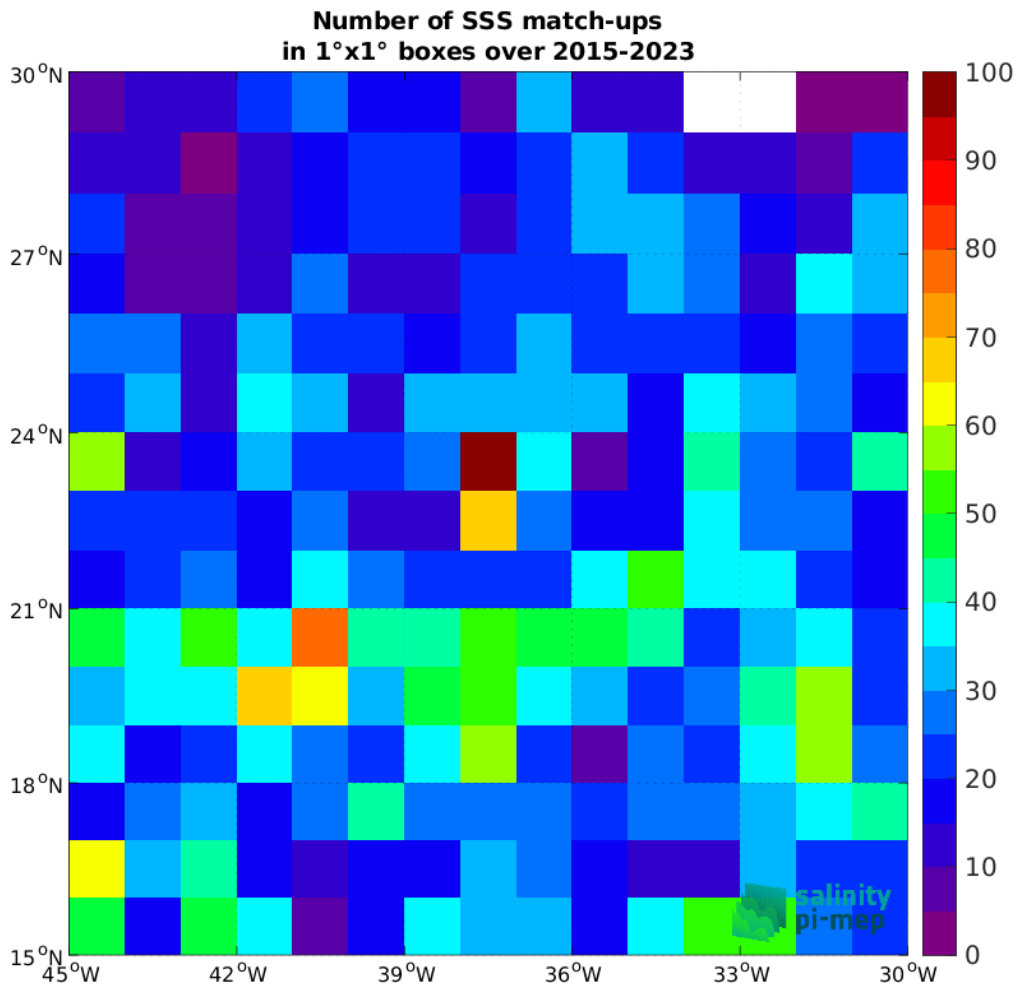
Figure 5: Number of SSS match-ups between Argo SSS and the SMAP SSS L2 v5.3 (RSS) SSS product for the SPURS 1 Pi-MEP region over 1°×1° boxes and for the full satellite product period.
