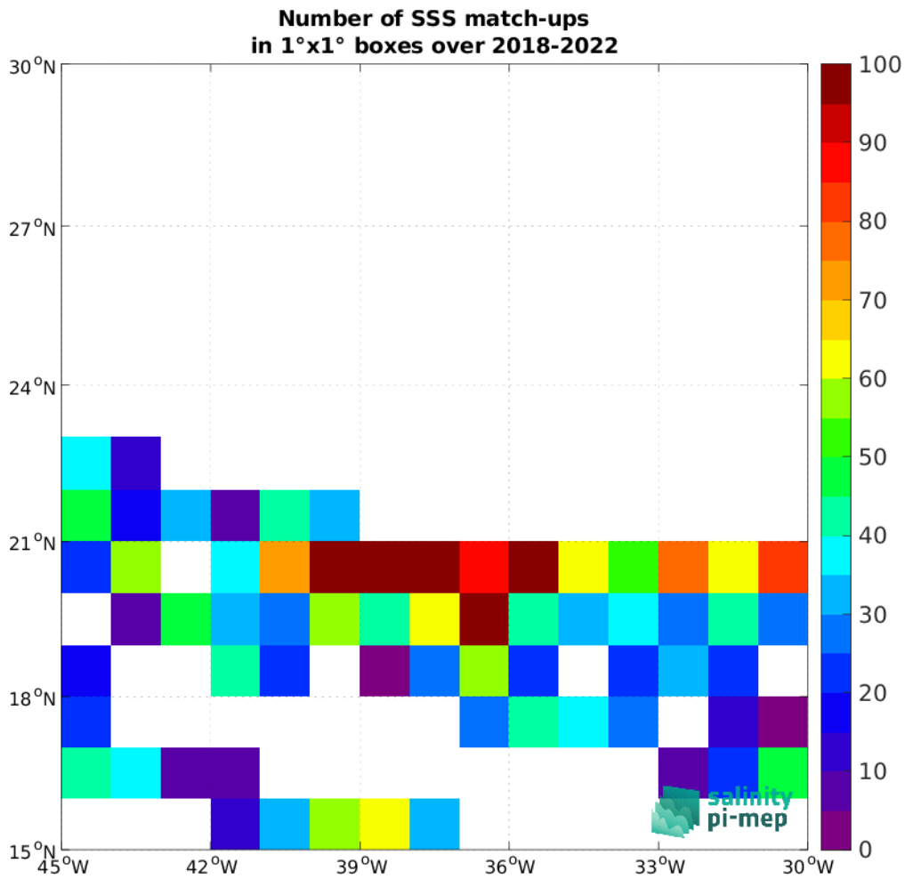
Figure 5: Number of SSS match-ups between TSG (SAMOS) SSS and the SMAP SSS L2 v5.3 - 40 km (RSS) SSS product for the SPURS 1 Pi-MEP region over 1^\circ \times 1^\circ boxes and for the full satellite product period.
