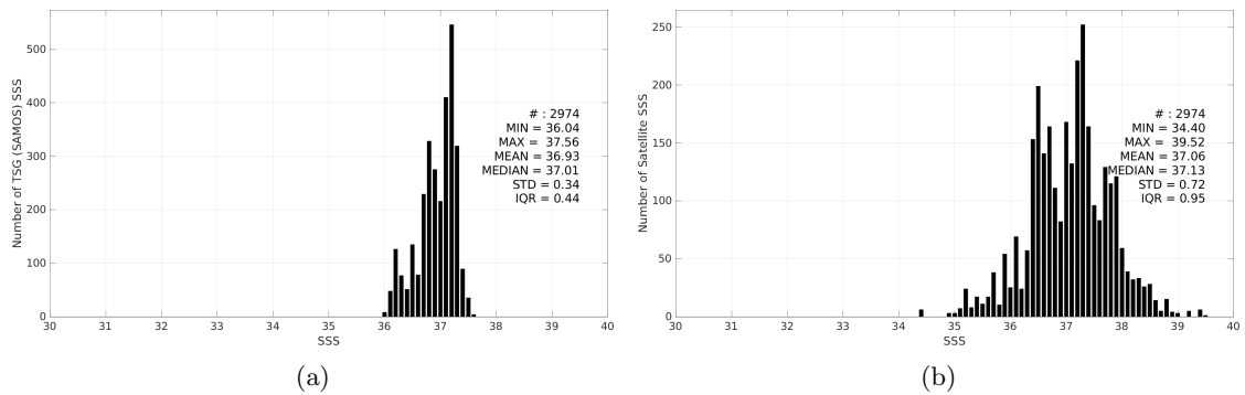
Figure 3: Histograms of SSS from TSG (SAMOS) (a) and SMAP SSS L2 v5.3 - 40 km (RSS) (b) considering all match-up pairs per bins of 0.1 over the SPURS 1 Pi-MEP region and for the full satellite product period.
