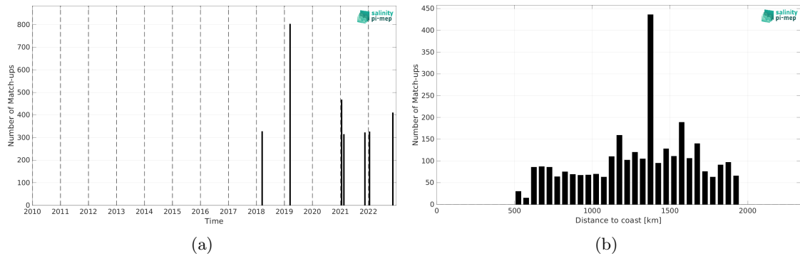
Figure 2: Number of match-ups between TSG (SAMOS) and SMAP SSS L2 v5.3 - 40 km (RSS) SSS as a function of time (a) and as function of the distance to coast (b) over the SPURS 1 Pi-MEP region and for the full satellite product period.
