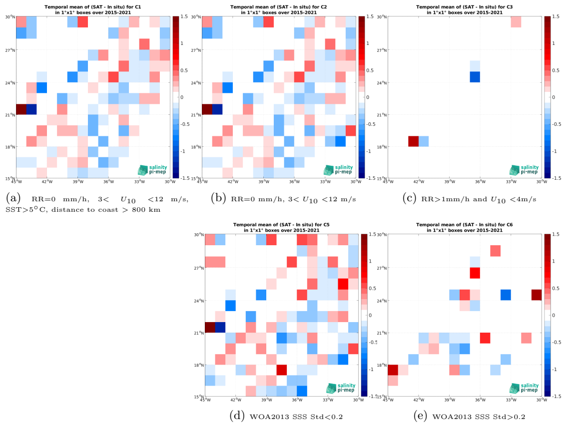
Figure 14: Temporal mean gridded over spatial boxes of size 1^\circ \times 1^\circ of \Delta\text{SSS} (SMAP SSS L2 v5.3 - 40 km (RSS) - TSG (LEGOS-DM)) for 5 different subdatasets corresponding to:RR=0 mm/h, 3 < U_{10} < 12 m/s, SST > 5^\circ\text{C} , distance to coast > 800 km (a), RR=0 mm/h, 3 < U_{10} < 12 m/s (b), RR > 1 mm/h and U_{10} < 4 m/s (c), WOA2013 SSS Std < 0.2 (d), WOA2013 SSS Std > 0.2 (e).
