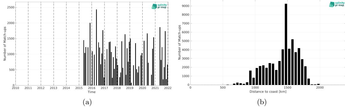
Figure 2: Number of match-ups between TSG (LEGOS-DM) and SMAP SSS L2 v5.3 - 40 km (RSS) SSS as a function of time (a) and as function of the distance to coast (b) over the SPURS 1 Pi-MEP region and for the full satellite product period.
