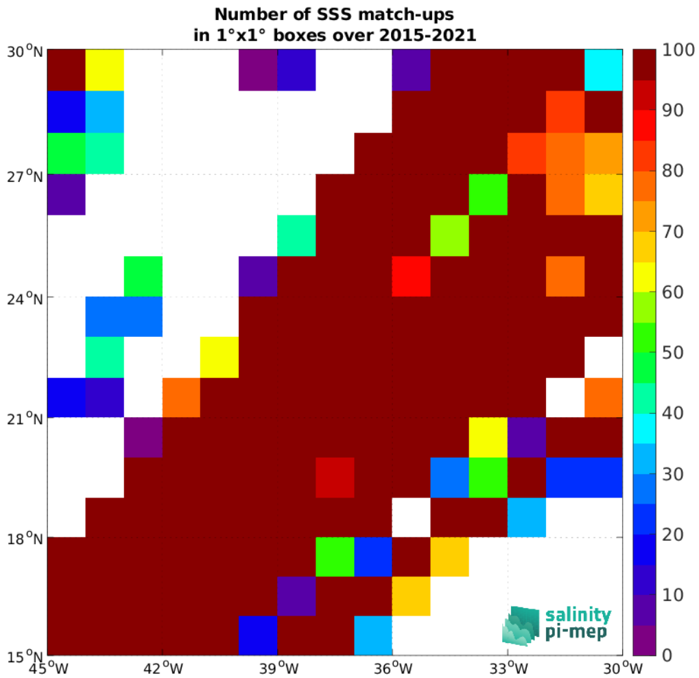
Figure 5: Number of SSS match-ups between TSG (LEGOS-DM) SSS and the SMAP SSS L2 v5.3 - 40 km (RSS) SSS product for the SPURS 1 Pi-MEP region over 1^\circ \times 1^\circ boxes and for the full satellite product period.
