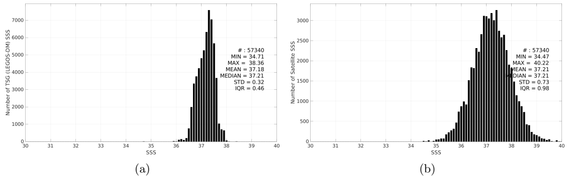
Figure 3: Histograms of SSS from TSG (LEGOS-DM) (a) and SMAP SSS L2 v5.3 - 40 km (RSS) (b) considering all match-up pairs per bins of 0.1 over the SPURS 1 Pi-MEP region and for the full satellite product period.
