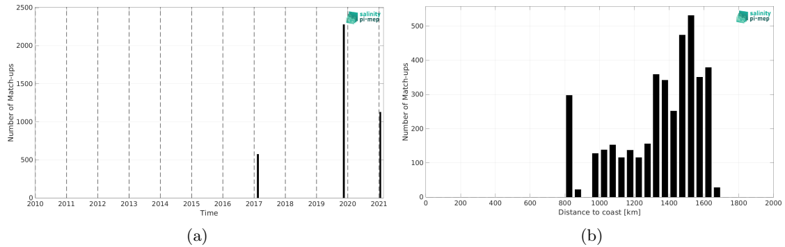
Figure 2: Number of match-ups between TSG (GOSUD-Sailing-ship) and SMAP SSS L2 v5.3 - 40 km (RSS) SSS as a function of time (a) and as function of the distance to coast (b) over the SPURS 1 Pi-MEP region and for the full satellite product period.
