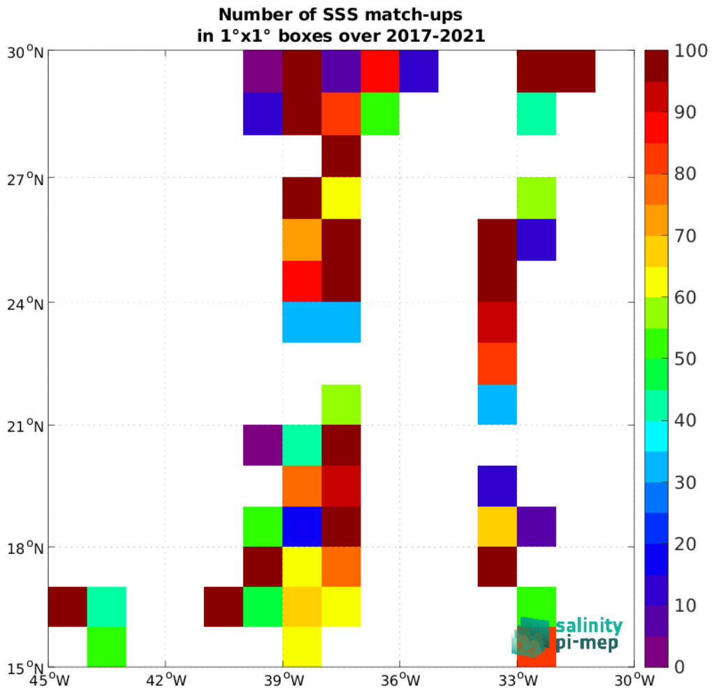
Figure 5: Number of SSS match-ups between TSG (GOSUD-Sailing-ship) SSS and the SMAP SSS L2 v5.3 - 40 km (RSS) SSS product for the SPURS 1 Pi-MEP region over 1^\circ \times 1^\circ boxes and for the full satellite product period.
