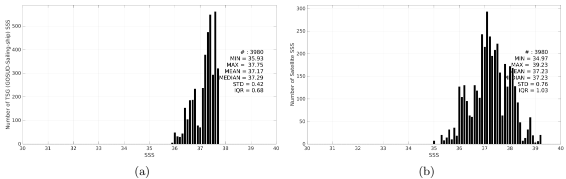
Figure 3: Histograms of SSS from TSG (GOSUD-Sailing-ship) (a) and SMAP SSS L2 v5.3 - 40 km (RSS) (b) considering all match-up pairs per bins of 0.1 over the SPURS 1 Pi-MEP region and for the full satellite product period.
