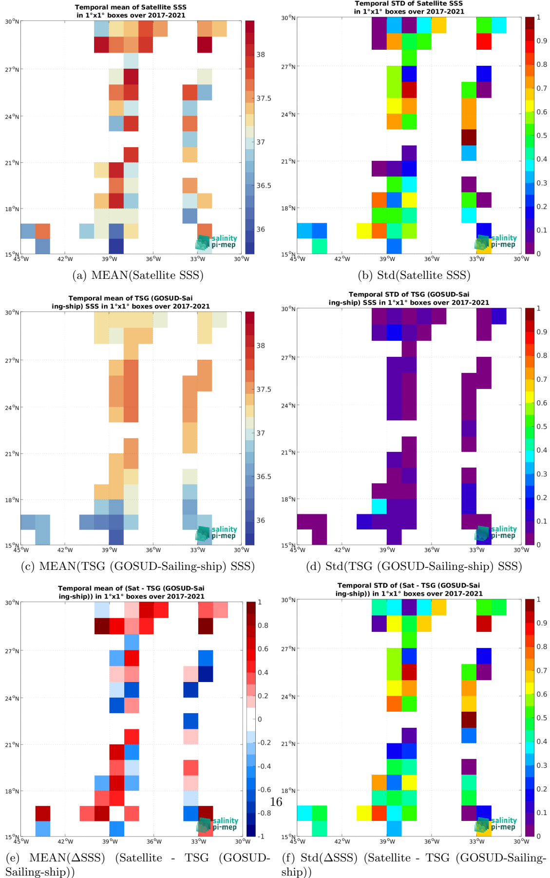
Figure 7: Temporal mean (left) and Std (right) of SSS from SMAP SSS L2 v5.3 - 40 km (RSS) (top), TSG (GOSUD-Sailing-ship) (middle), and of \Delta SSS (Satellite - TSG (GOSUD-Sailing-ship)). Only match-up pairs are used to generate these maps.
