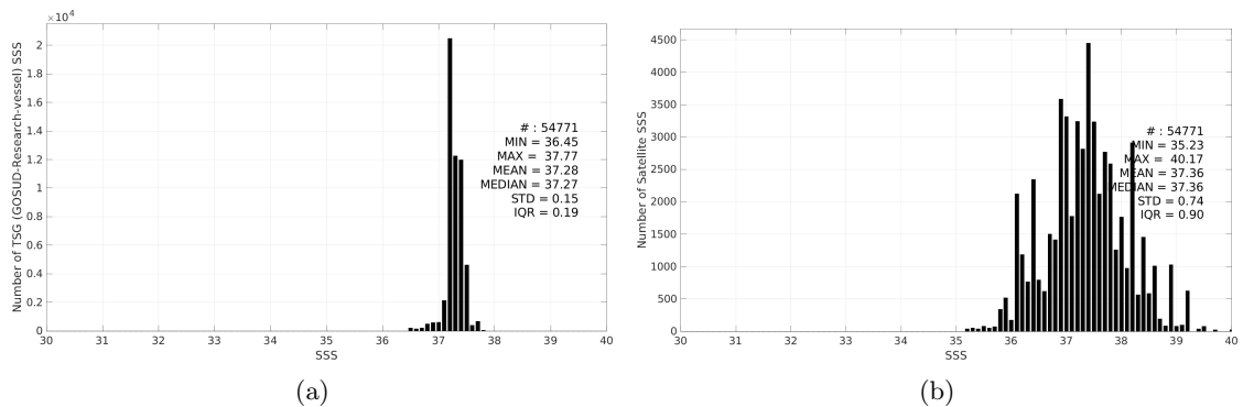
Figure 3: Histograms of SSS from TSG (GOSUD-Research-vessel) (a) and SMAP SSS L2 v5.3 - 40 km (RSS) (b) considering all match-up pairs per bins of 0.1 over the SPURS 1 Pi-MEP region and for the full satellite product period.
