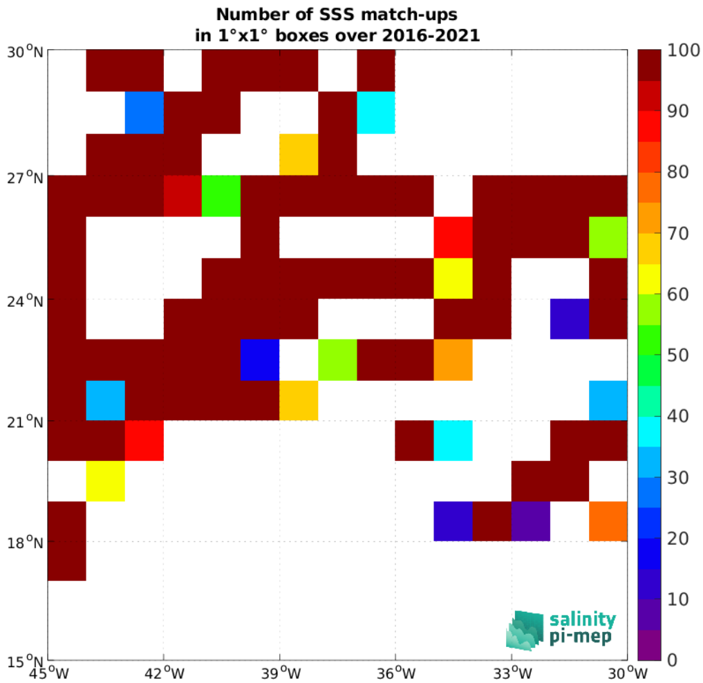
Figure 5: Number of SSS match-ups between TSG (GOSUD-Research-vessel) SSS and the SMAP SSS L2 v5.3 - 40 km (RSS) SSS product for the SPURS 1 Pi-MEP region over 1°x1° boxes and for the full satellite product period.
