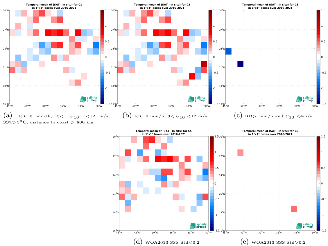
Figure 14: Temporal mean gridded over spatial boxes of size 1^\circ \times 1^\circ of \Delta SSS (SMAP SSS L2 v5.3 - 40 km (RSS) - TSG (GOSUD-Research-vessel)) for 5 different subdatasets corresponding to:RR=0 mm/h, 3 < U_{10} < 12 m/s, SST>5°C, distance to coast > 800 km (a), RR=0 mm/h, 3 < U_{10} < 12 m/s (b), RR>1mm/h and U_{10} < 4 m/s (c), WOA2013 SSS Std<0.2 (d), WOA2013 SSS Std>0.2 (e).
