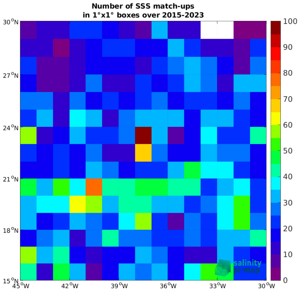
Figure 5: Number of SSS match-ups between Argo SSS and the SMAP SSS L2 v5.3 - 40 km (RSS) SSS product for the SPURS 1 Pi-MEP region over 1°x1° boxes and for the full satellite product period.
