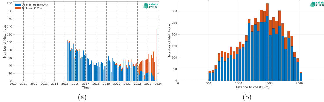
Figure 2: Number of match-ups between Argo and SMAP SSS L2 v5.3 - 40 km (RSS) SSS as a function of time (a) and as function of the distance to coast (b) over the SPURS 1 Pi-MEP region and for the full satellite product period.
