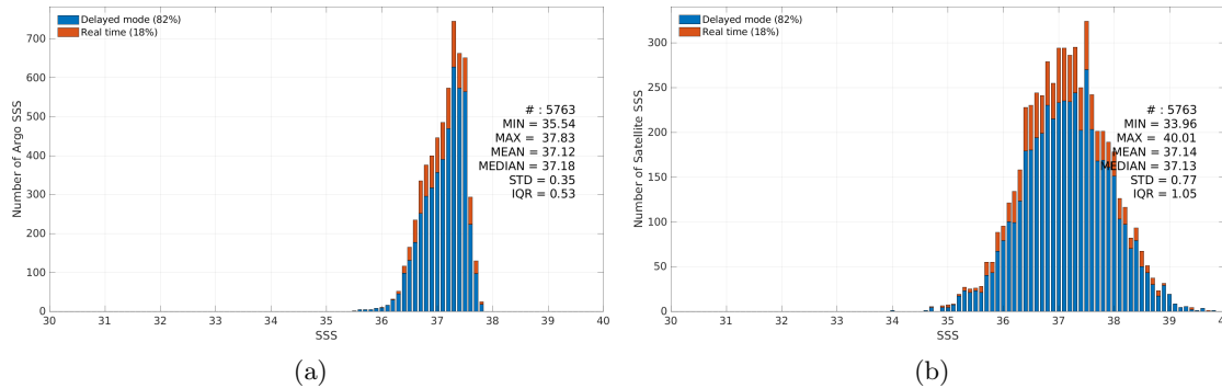
Figure 3: Histograms of SSS from Argo (a) and SMAP SSS L2 v5.3 - 40 km (RSS) (b) considering all match-up pairs per bins of 0.1 over the SPURS 1 Pi-MEP region and for the full satellite product period.
