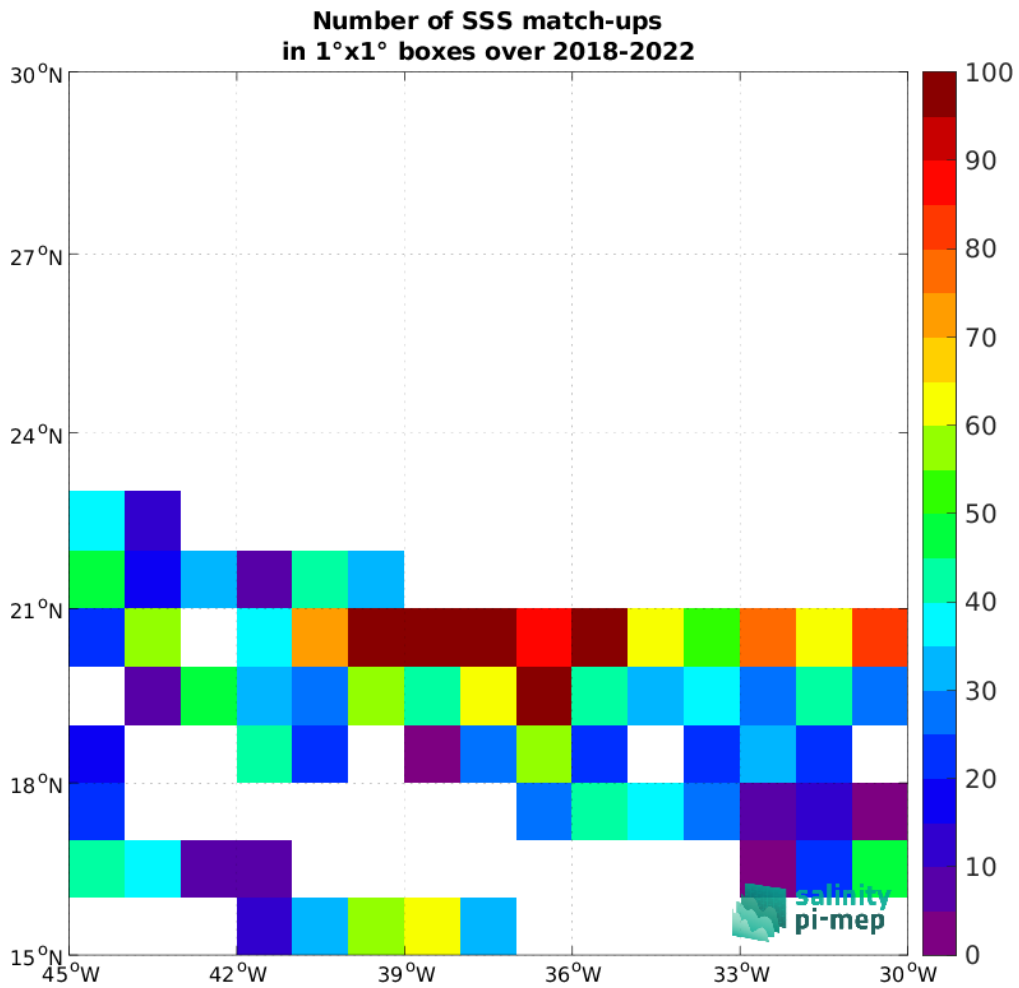
Figure 4: Number of SSS match-ups between TSG (SAMOS) SSS and the SMAP SSS L2 v5 - 40 km (RSS) SSS product for the SPURS 1 Pi-MEP region over 1°x1° boxes and for the full satellite product period.
