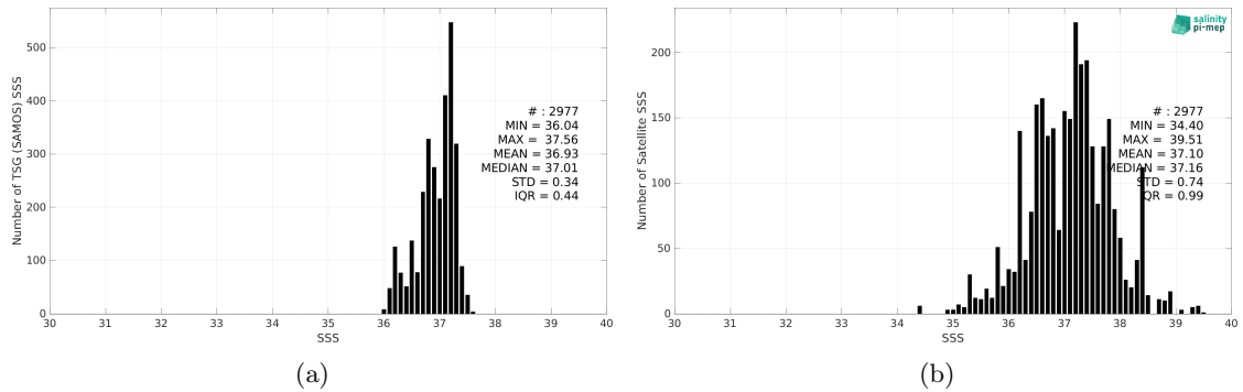
Figure 2: Histograms of SSS from TSG (SAMOS) (a) and SMAP SSS L2 v5 - 40 km (RSS) (b) considering all match-up pairs per bins of 0.1 over the SPURS 1 Pi-MEP region and for the full satellite product period.
