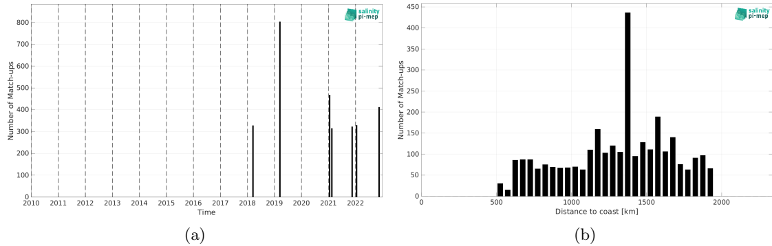
Figure 1: Number of match-ups between TSG (SAMOS) and SMAP SSS L2 v5 - 40 km (RSS) SSS as a function of time (a) and as function of the distance to coast (b) over the SPURS 1 Pi-MEP region and for the full satellite product period.
