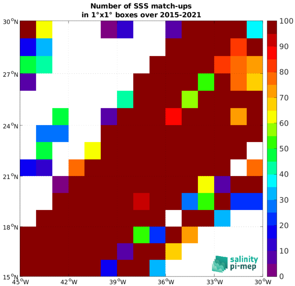
Figure 4: Number of SSS match-ups between TSG (LEGOS-DM) SSS and the SMAP SSS L2 v5 - 40 km (RSS) SSS product for the SPURS 1 Pi-MEP region over 1^\circ \times 1^\circ boxes and for the full satellite product period.
