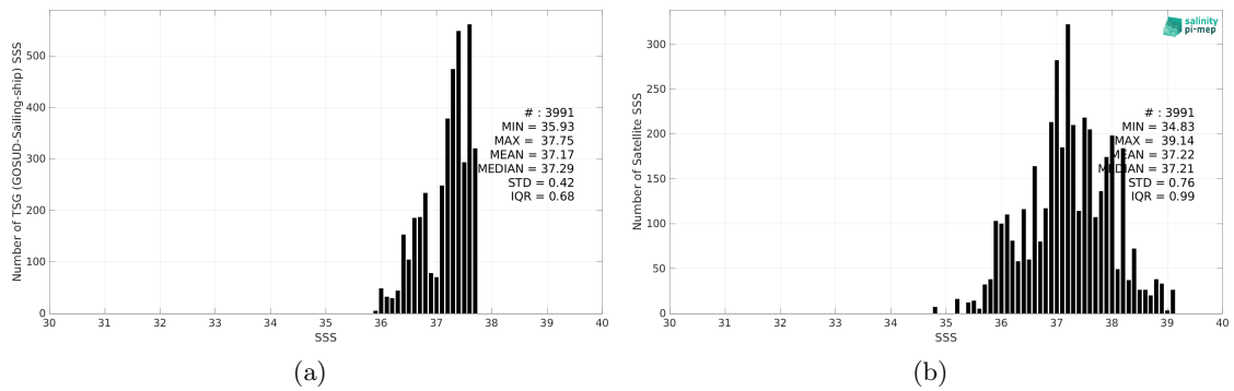
Figure 2: Histograms of SSS from TSG (GOSUD-Sailing-ship) (a) and SMAP SSS L2 v5 - 40 km (RSS) (b) considering all match-up pairs per bins of 0.1 over the SPURS 1 Pi-MEP region and for the full satellite product period.
