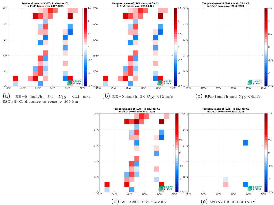
Figure 12: Temporal mean gridded over spatial boxes of size 1^\circ \times 1^\circ of \Delta SSS (SMAP SSS L2 v5 - 40 km (RSS) - TSG (GOSUD-Sailing-ship)) for 5 different subdatasets corresponding to:RR=0 mm/h, 3 < U_{10} < 12 m/s, SST>5°C, distance to coast > 800 km (a), RR=0 mm/h, 3 < U_{10} < 12 m/s (b), RR>1mm/h and U_{10} < 4 m/s (c), WOA2013 SSS Std<0.2 (d), WOA2013 SSS Std>0.2 (e).
