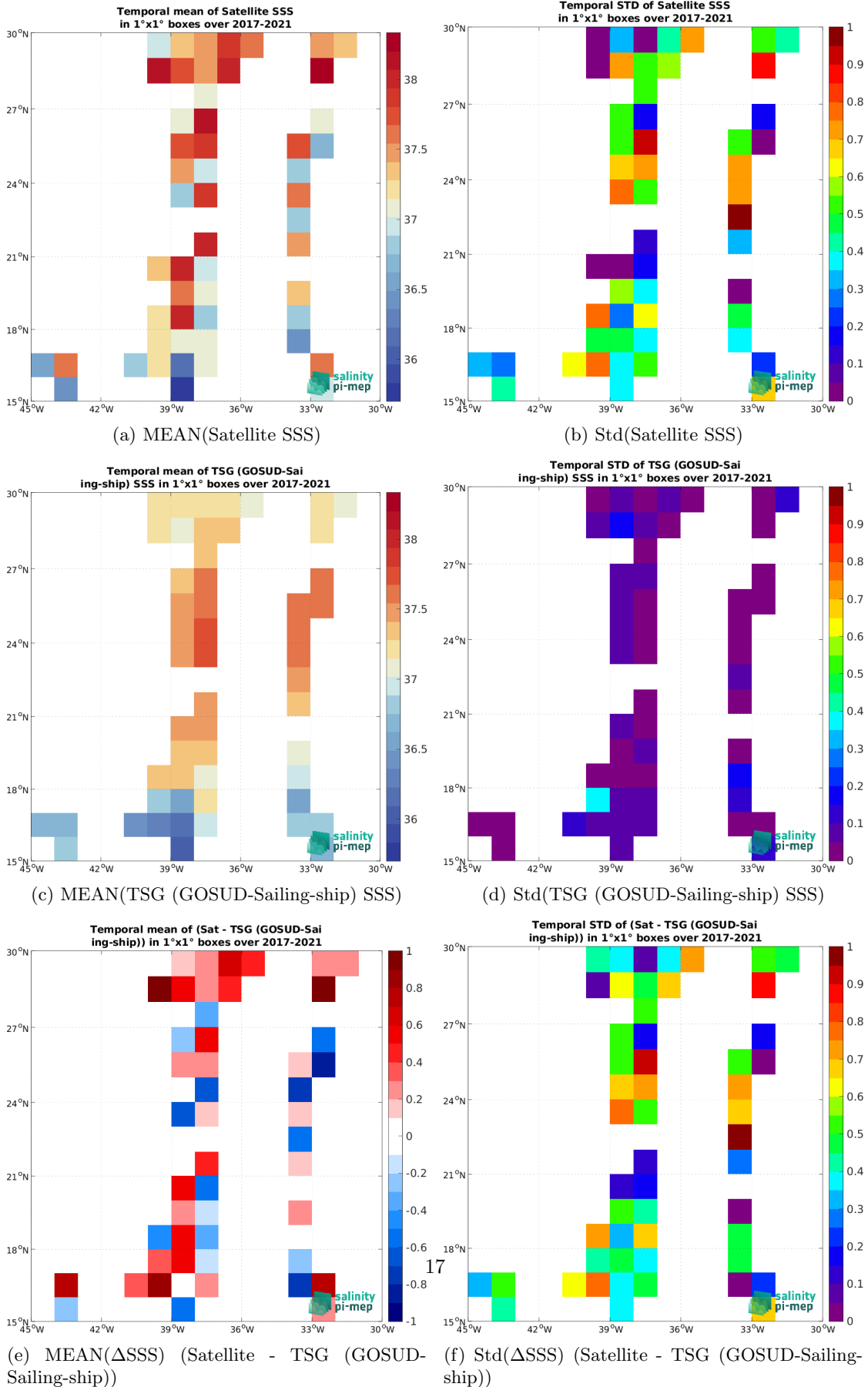
Figure 6: Temporal mean (left) and Std (right) of SSS from SMAP SSS L2 v5 - 40 km (RSS) (top), TSG (GOSUD-Sailing-ship) (middle), and of \Delta SSS (Satellite - TSG (GOSUD-Sailing-ship)). Only match-up pairs are used to generate these maps.
