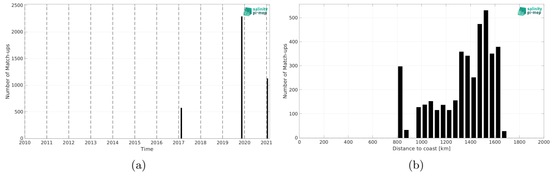
Figure 1: Number of match-ups between TSG (GOSUD-Sailing-ship) and SMAP SSS L2 v5 - 40 km (RSS) SSS as a function of time (a) and as function of the distance to coast (b) over the SPURS 1 Pi-MEP region and for the full satellite product period.
