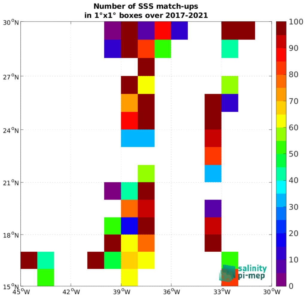
Figure 4: Number of SSS match-ups between TSG (GOSUD-Sailing-ship) SSS and the SMAP SSS L2 v5 - 40 km (RSS) SSS product for the SPURS 1 Pi-MEP region over 1°×1° boxes and for the full satellite product period.
