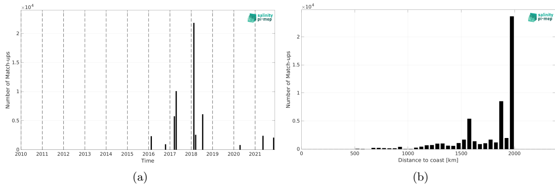
Figure 1: Number of match-ups between TSG (GOSUD-Research-vessel) and SMAP SSS L2 v5 - 40 km (RSS) SSS as a function of time (a) and as function of the distance to coast (b) over the SPURS 1 Pi-MEP region and for the full satellite product period.
