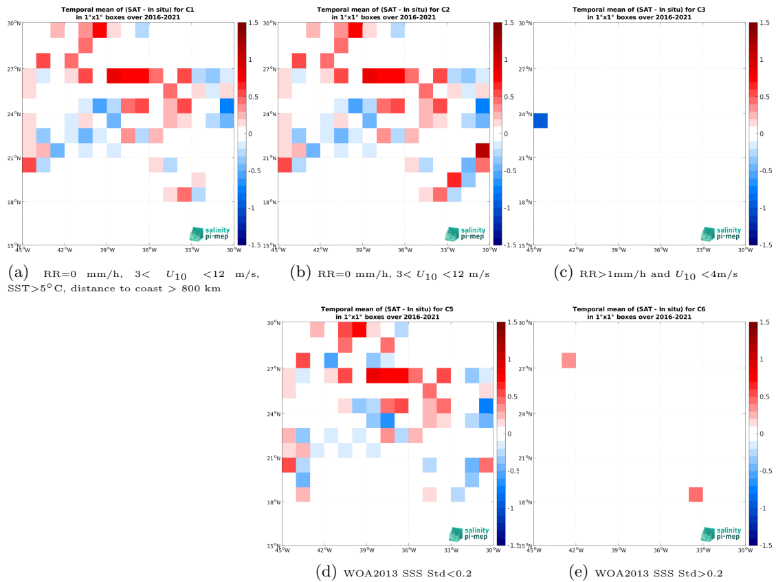
Figure 12: Temporal mean gridded over spatial boxes of size 1^\circ \times 1^\circ of \Delta SSS (SMAP SSS L2 v5 - 40 km (RSS) - TSG (GOSUD-Research-vessel)) for 5 different subdatasets corresponding to:RR=0 mm/h, 3 < U_{10} < 12 m/s, SST>5°C, distance to coast > 800 km (a), RR=0 mm/h, 3 < U_{10} < 12 m/s (b), RR>1mm/h and U_{10} < 4 m/s (c), WOA2013 SSS Std<0.2 (d), WOA2013 SSS Std>0.2 (e).
