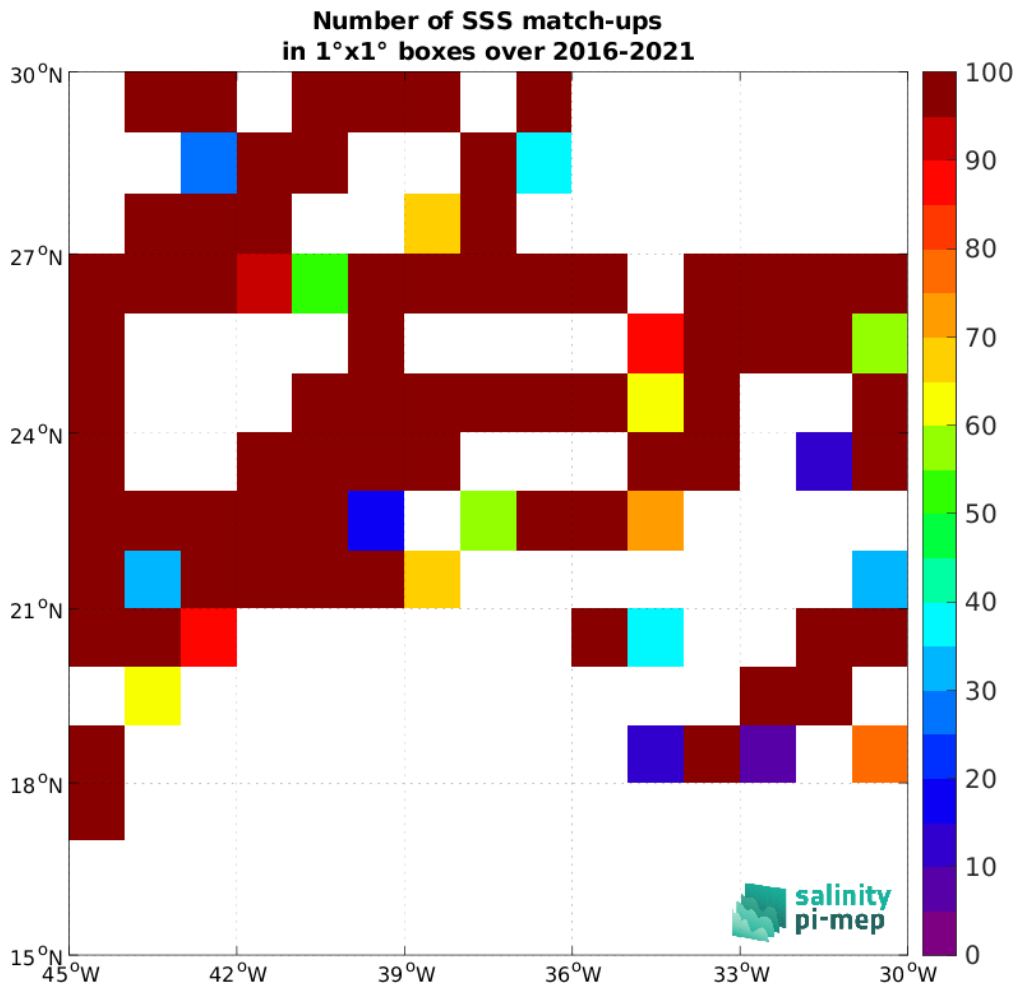
Figure 4: Number of SSS match-ups between TSG (GOSUD-Research-vessel) SSS and the SMAP SSS L2 v5 - 40 km (RSS) SSS product for the SPURS 1 Pi-MEP region over 1°×1° boxes and for the full satellite product period.
