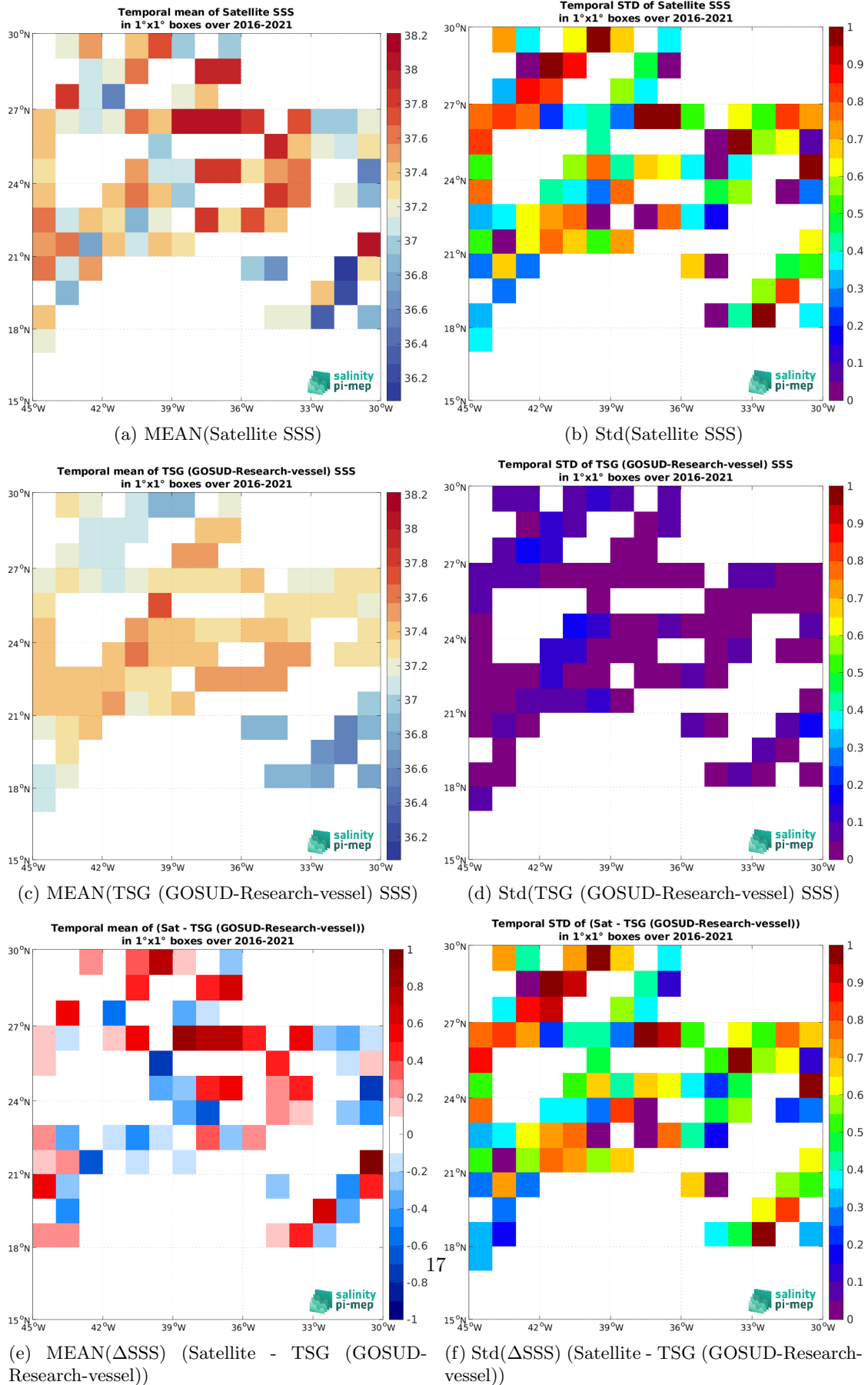
Figure 6: Temporal mean (left) and Std (right) of SSS from SMAP SSS L2 v5 - 40 km (RSS) (top), TSG (GOSUD-Research-vessel) (middle), and of \Delta SSS (Satellite - TSG (GOSUD-Research-vessel)). Only match-up pairs are used to generate these maps.
