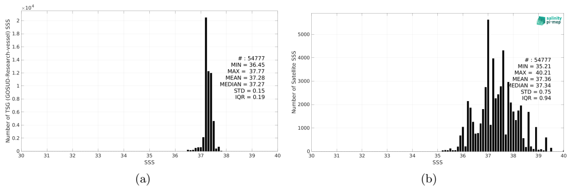
Figure 2: Histograms of SSS from TSG (GOSUD-Research-vessel) (a) and SMAP SSS L2 v5 - 40 km (RSS) (b) considering all match-up pairs per bins of 0.1 over the SPURS 1 Pi-MEP region and for the full satellite product period.
