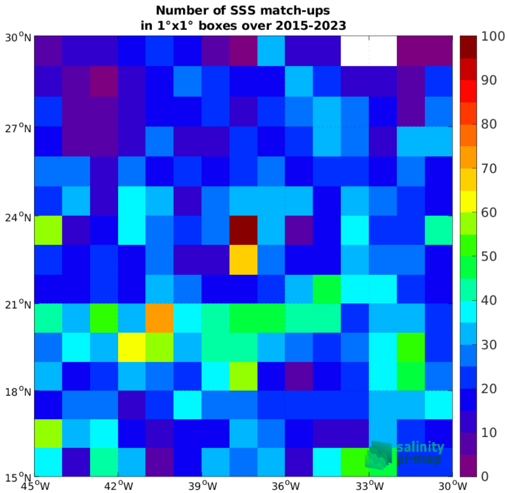
Figure 4: Number of SSS match-ups between Argo SSS and the SMAP SSS L2 v5 - 40 km (RSS) SSS product for the SPURS 1 Pi-MEP region over 1°×1° boxes and for the full satellite product period.
