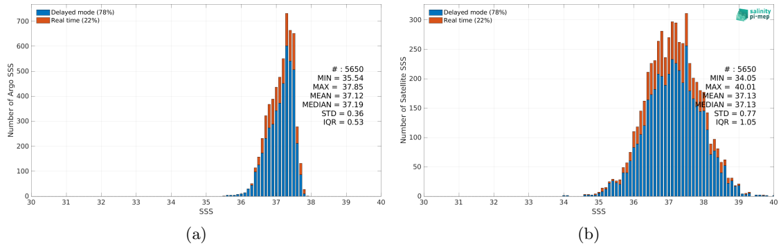
Figure 2: Histograms of SSS from Argo (a) and SMAP SSS L2 v5 - 40 km (RSS) (b) considering all match-up pairs per bins of 0.1 over the SPURS 1 Pi-MEP region and for the full satellite product period.
