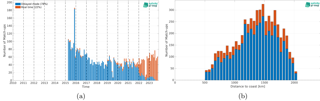
Figure 1: Number of match-ups between Argo and SMAP SSS L2 v5 - 40 km (RSS) SSS as a function of time (a) and as function of the distance to coast (b) over the SPURS 1 Pi-MEP region and for the full satellite product period.
