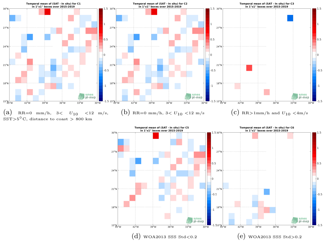
Figure 12: Temporal mean gridded over spatial boxes of size 1^\circ \times 1^\circ of \Delta SSS (SMAP SSS L2 v4 (RSS) - TSG (LEGOS-DM)) for 5 different subdatasets corresponding to: RR=0 mm/h, 3 < U_{10} < 12 m/s, SST > 5^\circ C , distance to coast > 800 km (a), RR=0 mm/h, 3 < U_{10} < 12 m/s (b), RR > 1 mm/h and U_{10} < 4 m/s (c), WOA2013 SSS Std < 0.2 (d), WOA2013 SSS Std > 0.2 (e).
