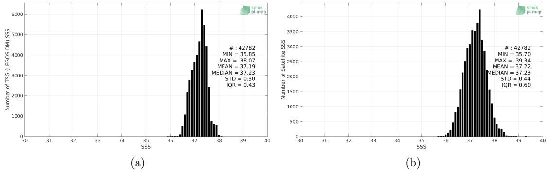
Figure 2: Histograms of SSS from TSG (LEGOS-DM) (a) and SMAP SSS L2 v4 (RSS) (b) considering all match-up pairs per bins of 0.1 over the SPURS 1 Pi-MEP region and for the full satellite product period.
