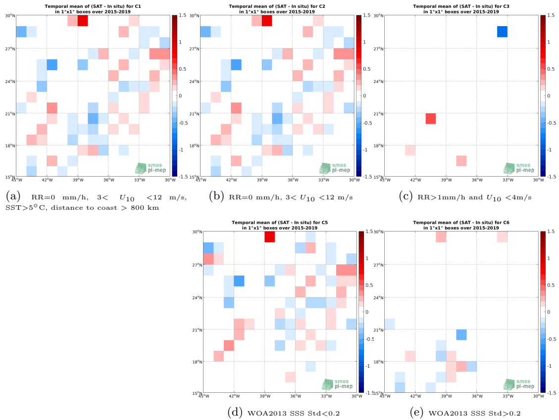
Figure 12: Temporal mean gridded over spatial boxes of size 1^\circ \times 1^\circ of \Delta\text{SSS} (SMAP SSS L2 v4 (RSS) - TSG (LEGOS-DM)) for 5 different subdatasets corresponding to:RR=0 mm/h, 3 < U_{10} < 12 m/s, SST >5^\circ\text{C} , distance to coast > 800 km (a), RR=0 mm/h, 3 < U_{10} < 12 m/s (b), RR >1 mm/h and U_{10} < 4 m/s (c), WOA2013 SSS Std <0.2 (d), WOA2013 SSS Std >0.2 (e).
