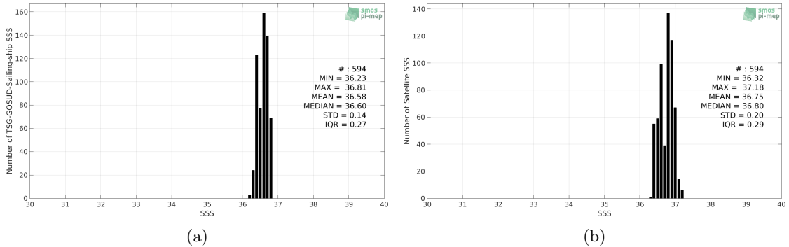
Figure 2: Histograms of SSS from TSG-GOSUD-Sailing-ship (a) and SMAP-L2-RSS-V4 (b) considering all match-up pairs per bins of 0.1 over the SPURS 1 Pi-MEP region and for the full satellite product period.
