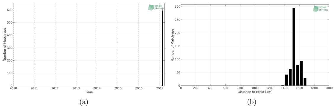
Figure 1: Number of match-ups between TSG-GOSUD-Sailing-ship and SMAP-L2-RSS-V4 SSS as a function of time (a) and as function of the distance to coast (b) over the SPURS 1 Pi-MEP region and for the full satellite product period.
