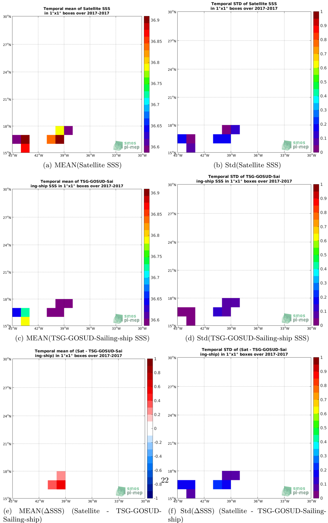
Figure 6: Temporal mean (left) and Std (right) of SSS from SMAP-L2-RSS-V4 (top), TSG-GOSUD-Sailing-ship (middle), and of \Delta SSS (Satellite - TSG-GOSUD-Sailing-ship). Only match-up pairs are used to generate these maps.
