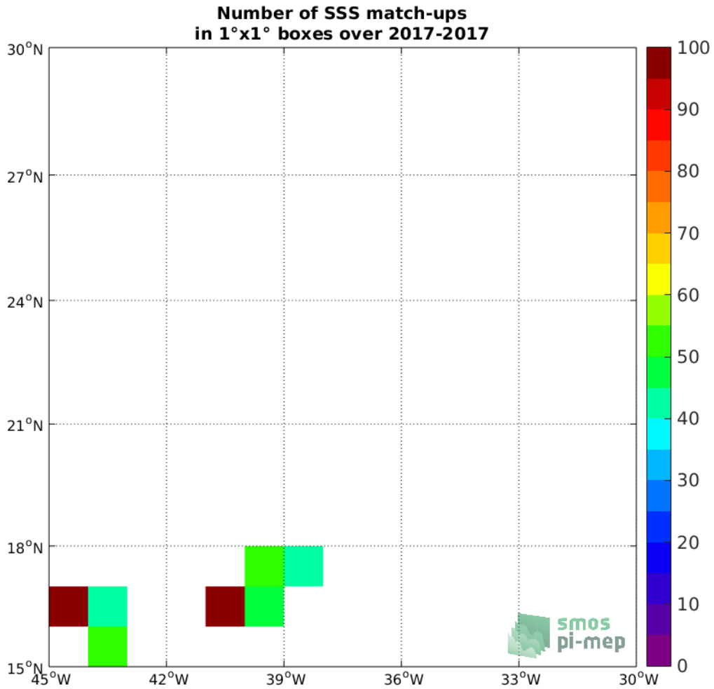
Figure 4: Number of SSS match-ups between TSG-GOSUD-Sailing-ship SSS and the SMAP-L2-RSS-V4 SSS product for the SPURS 1 Pi-MEP region over 1°x1° boxes and for the full satellite product period.
