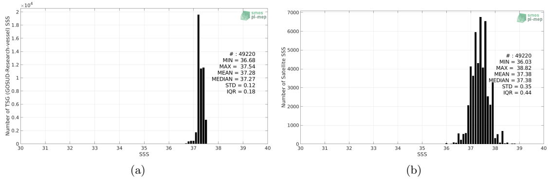
Figure 2: Histograms of SSS from TSG (GOSUD-Research-vessel) (a) and SMAP SSS L2 v4 (RSS) (b) considering all match-up pairs per bins of 0.1 over the SPURS 1 Pi-MEP region and for the full satellite product period.
