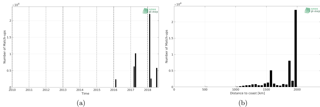
Figure 1: Number of match-ups between TSG (GOSUD-Research-vessel) and SMAP SSS L2 v4 (RSS) SSS as a function of time (a) and as function of the distance to coast (b) over the SPURS 1 Pi-MEP region and for the full satellite product period.
