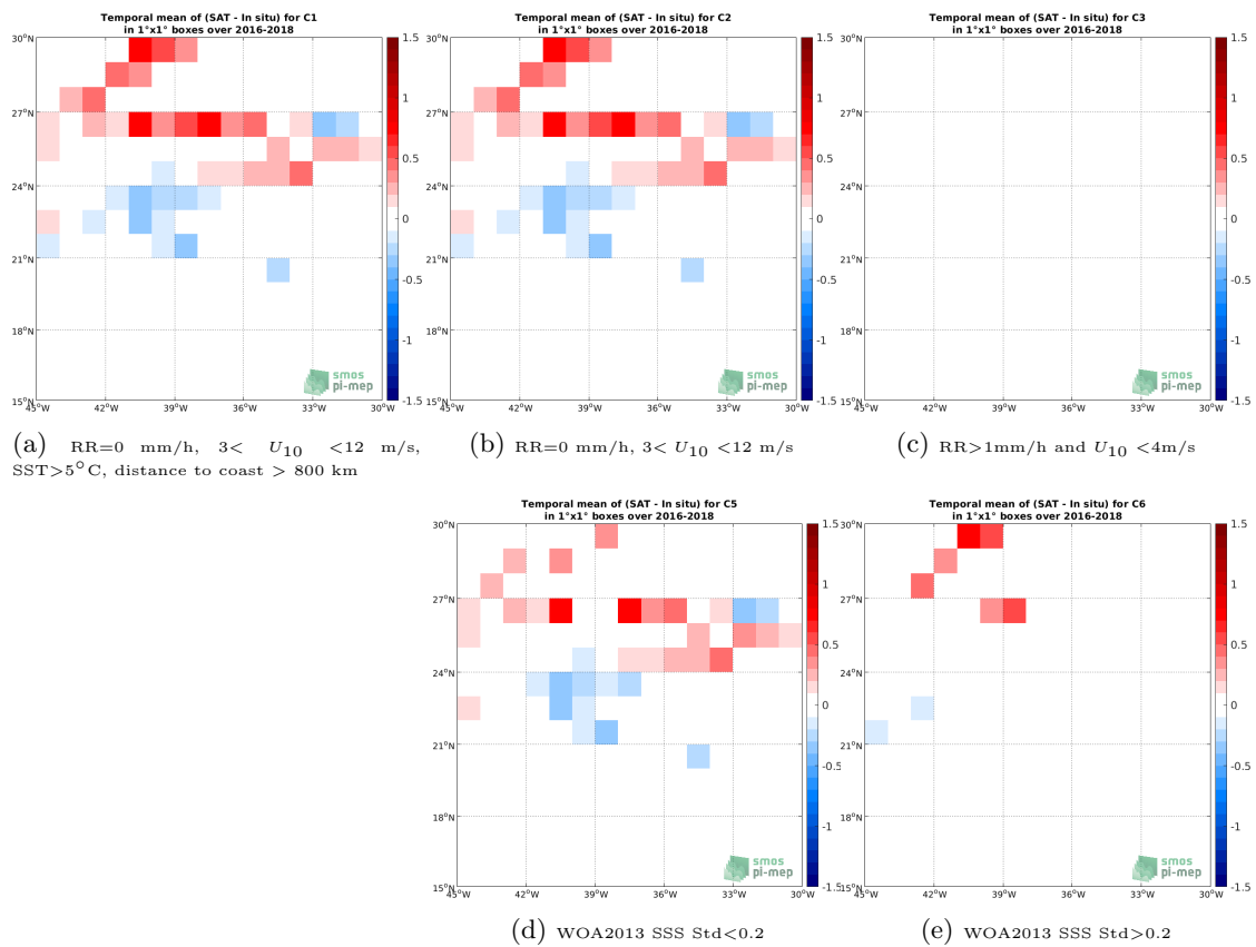
Figure 12: Temporal mean gridded over spatial boxes of size 1^\circ \times 1^\circ of \Delta\text{SSS} (SMAP SSS L2 v4 (RSS) - TSG (GOSUD-Research-vessel)) for 5 different subdatasets corresponding to:RR=0 mm/h, 3 < U_{10} < 12 m/s, SST>5°C, distance to coast > 800 km (a), RR=0 mm/h, 3 < U_{10} < 12 m/s (b), RR>1mm/h and U_{10} < 4 m/s (c), WOA2013 SSS Std<0.2 (d), WOA2013 SSS Std>0.2 (e).
