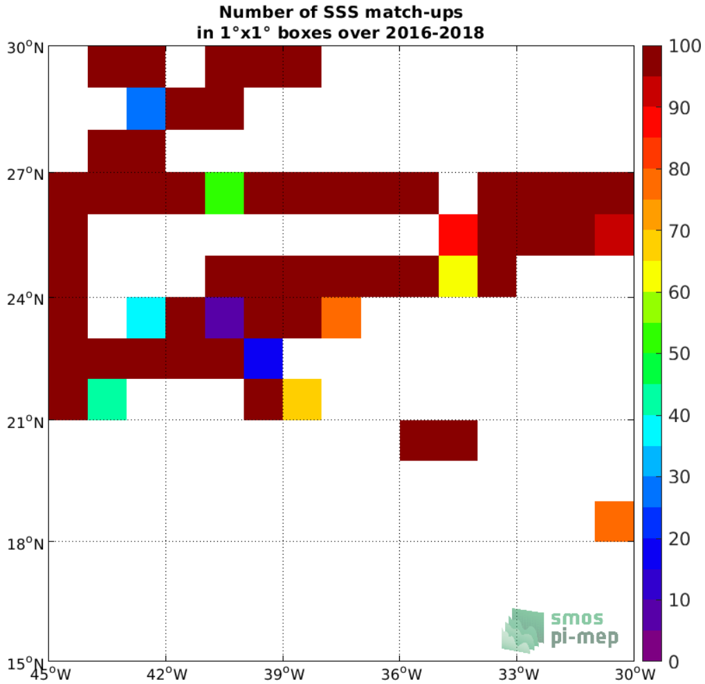
Figure 4: Number of SSS match-ups between TSG (GOSUD-Research-vessel) SSS and the SMAP SSS L2 v4 (RSS) SSS product for the SPURS 1 Pi-MEP region over 1°x1° boxes and for the full satellite product period.
