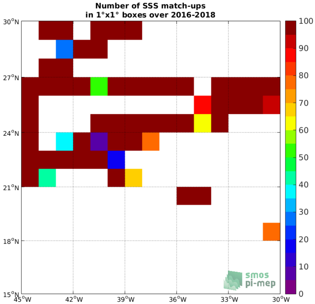
Figure 4: Number of SSS match-ups between TSG-GOSUD-Research-vessel SSS and the SMAP-L2-RSS-V4 SSS product for the SPURS 1 Pi-MEP region over 1°x1° boxes and for the full satellite product period.
