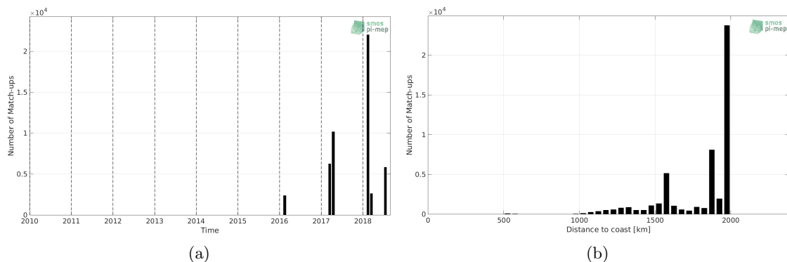
Figure 1: Number of match-ups between TSG-GOSUD-Research-vessel and SMAP-L2-RSS-V4 SSS as a function of time (a) and as function of the distance to coast (b) over the SPURS 1 Pi-MEP region and for the full satellite product period.
