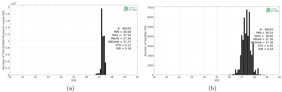
Figure 2: Histograms of SSS from TSG-GOSUD-Research-vessel (a) and SMAP-L2-RSS-V4 (b) considering all match-up pairs per bins of 0.1 over the SPURS 1 Pi-MEP region and for the full satellite product period.
