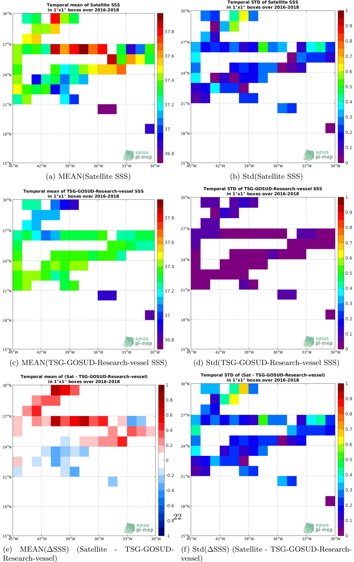
Figure 6: Temporal mean (left) and Std (right) of SSS from SMAP-L2-RSS-V4 (top), TSG-GOSUD-Research-vessel (middle), and of \Delta SSS (Satellite - TSG-GOSUD-Research-vessel). Only match-up pairs are used to generate these maps.
