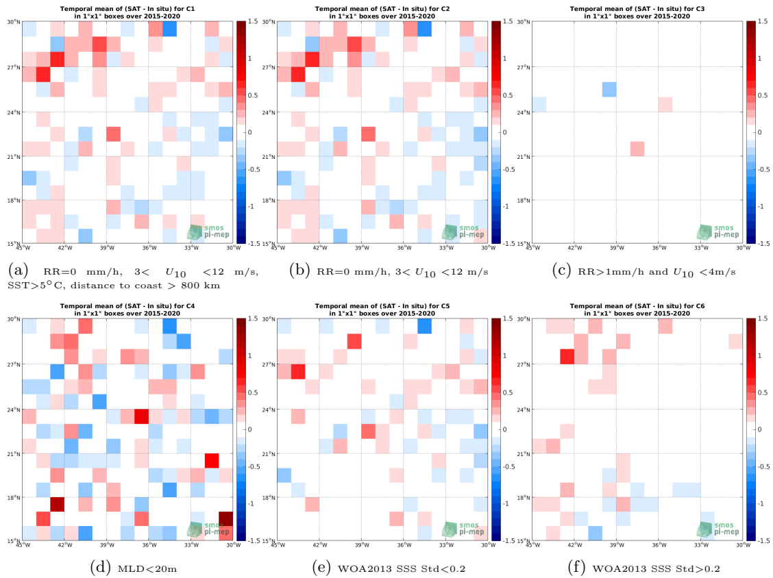
Figure 12: Temporal mean gridded over spatial boxes of size 1^\circ \times 1^\circ of \Delta SSS (SMAP SSS L2 v4 (RSS) - Argo) for 6 different subdatasets corresponding to: RR=0 mm/h, 3 < U_{10} < 12 m/s, SST >5^\circ C, distance to coast > 800 km (a), RR=0 mm/h, 3 < U_{10} < 12 m/s (b), RR >1 mm/h and U_{10} < 4 m/s (c),MLD <20 m (d),WOA2013 SSS Std <0.2 (e),WOA2013 SSS Std >0.2 (f).
