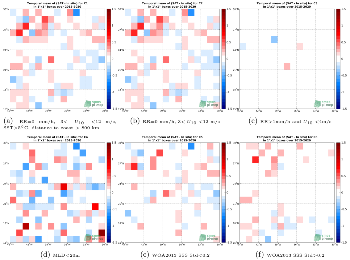
Figure 12: Temporal mean gridded over spatial boxes of size 1^\circ \times 1^\circ of \Delta SSS (SMAP-L2-RSS-V4 - Argo) for 6 different subdatasets corresponding to:RR=0 mm/h, 3 < U_{10} < 12 m/s, SST >5^\circ C, distance to coast > 800 km (a), RR=0 mm/h, 3 < U_{10} < 12 m/s (b), RR >1 mm/h and U_{10} < 4 m/s (c),MLD <20 m (d),WOA2013 SSS Std <0.2 (e),WOA2013 SSS Std >0.2 (f).
