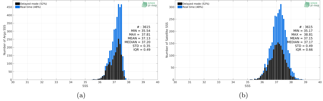
Figure 2: Histograms of SSS from Argo (a) and SMAP-L2-RSS-V4 (b) considering all match-up pairs per bins of 0.1 over the SPURS 1 Pi-MEP region and for the full satellite product period.
