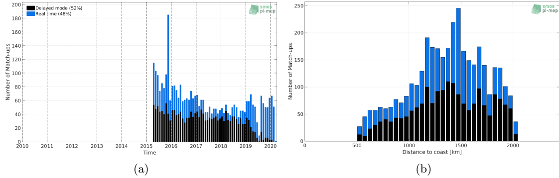
Figure 1: Number of match-ups between Argo and SMAP-L2-RSS-V4 SSS as a function of time (a) and as function of the distance to coast (b) over the SPURS 1 Pi-MEP region and for the full satellite product period.
