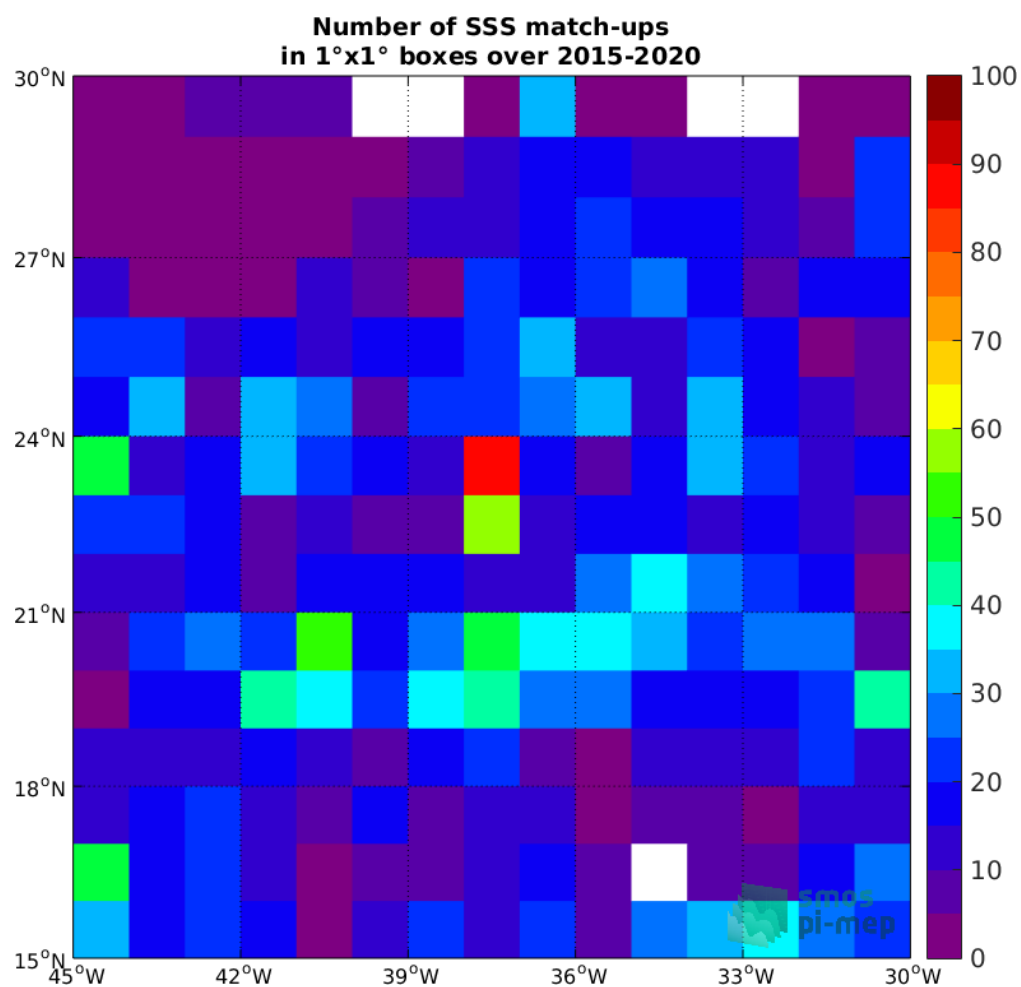
Figure 4: Number of SSS match-ups between Argo SSS and the SMAP-L2-RSS-V4 SSS product for the SPURS 1 Pi-MEP region over 1°x1° boxes and for the full satellite product period.
