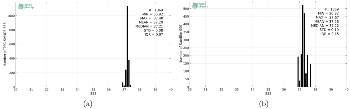
Figure 2: Histograms of SSS from TSG-SAMOS (a) and SMAP-L2-RSS-V3-70KM (b) considering all match-up pairs per bins of 0.1 over the SPURS 1 Pi-MEP region and for the full satellite product period.
