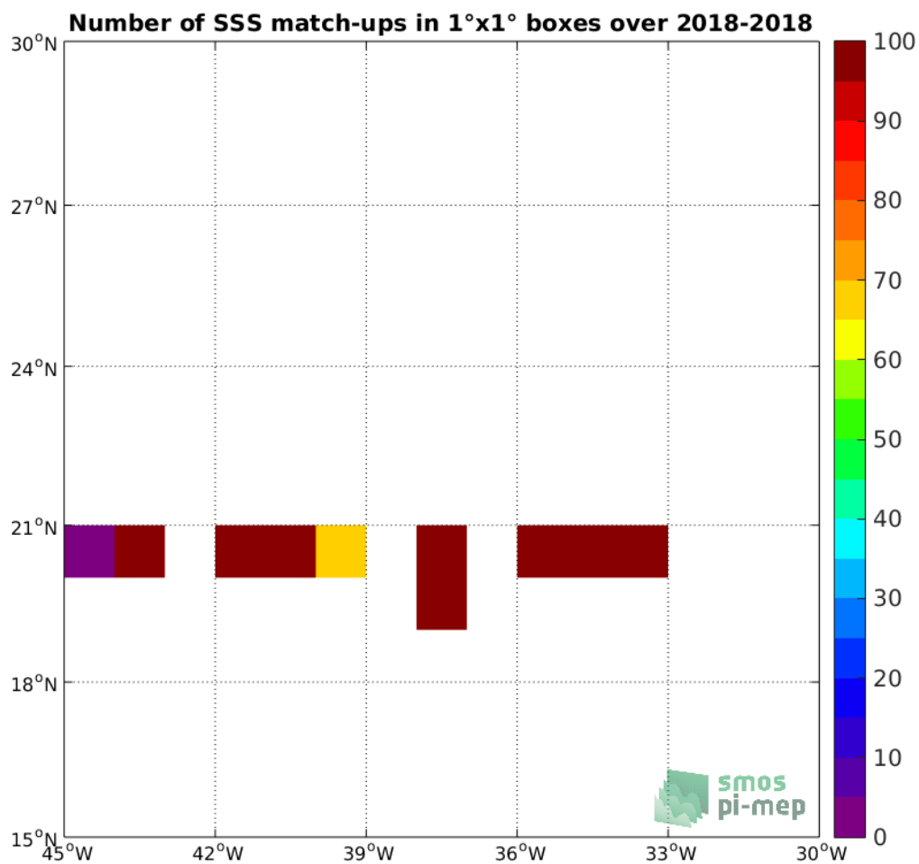
Figure 4: Number of SSS match-ups between TSG-SAMOS SSS and the SMAP-L2-RSS-V3-70KM SSS product for the SPURS 1 Pi-MEP region over 1°x1° boxes and for the full satellite product period.
