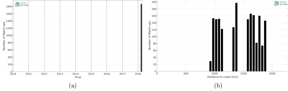
Figure 1: Number of match-ups between TSG-SAMOS and SMAP-L2-RSS-V3-70KM SSS as a function of time (a) and as function of the distance to coast (b) over the SPURS 1 Pi-MEP region and for the full satellite product period.
