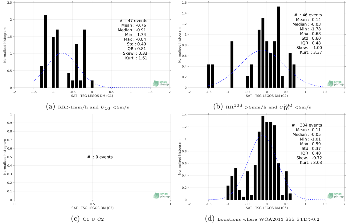
Figure 13: Normalized histogram of \Delta\text{SSS} (SMAP-L2-RSS-V3-70KM - TSG-LEGOS-DM) for 6 different subdatasets corresponding to: RR > 1\text{mm/h} and U_{10} < 5\text{m/s} (a), RR^{10d} > 5\text{mm/h} and U_{10}^{10d} < 5\text{m/s} (b), C1 \cup C2 (c), Locations where WOA2013 SSS STD > 0.2 (d).
