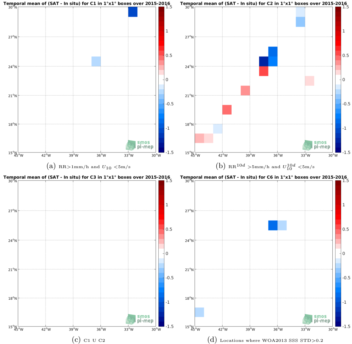
Figure 12: Temporal mean gridded over spatial boxes of size 1^\circ \times 1^\circ of \Delta SSS (SMAP-L2-RSS-V3-70KM - TSG-LEGOS-DM) for 4 different subdatasets corresponding to: RR > 1\text{mm/h} and U_{10} < 5\text{m/s} (a), RR^{10d} > 5\text{mm/h} and U_{10}^{10d} < 5\text{m/s} (b), C1 U C2 (c), Locations where WOA2013 SSS STD > 0.2 (d).
