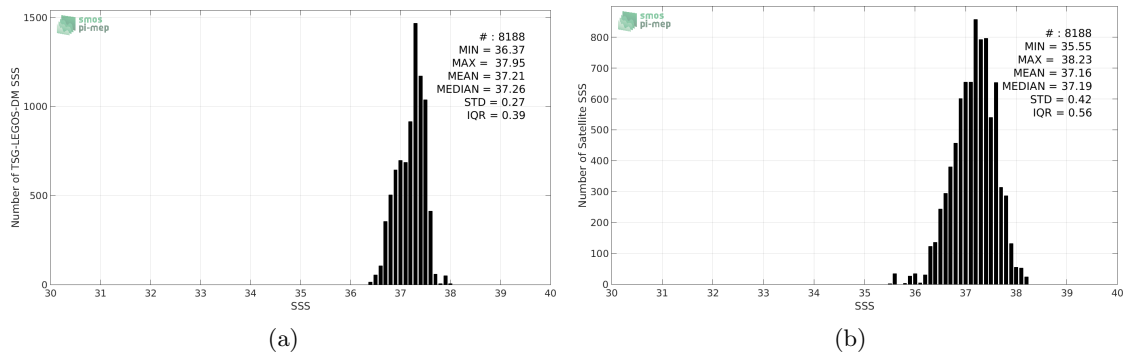
Figure 2: Histograms of SSS from TSG-LEGOS-DM (a) and SMAP-L2-RSS-V3-70KM (b) considering all match-up pairs per bins of 0.1 over the SPURS 1 Pi-MEP region and for the full satellite product period.
