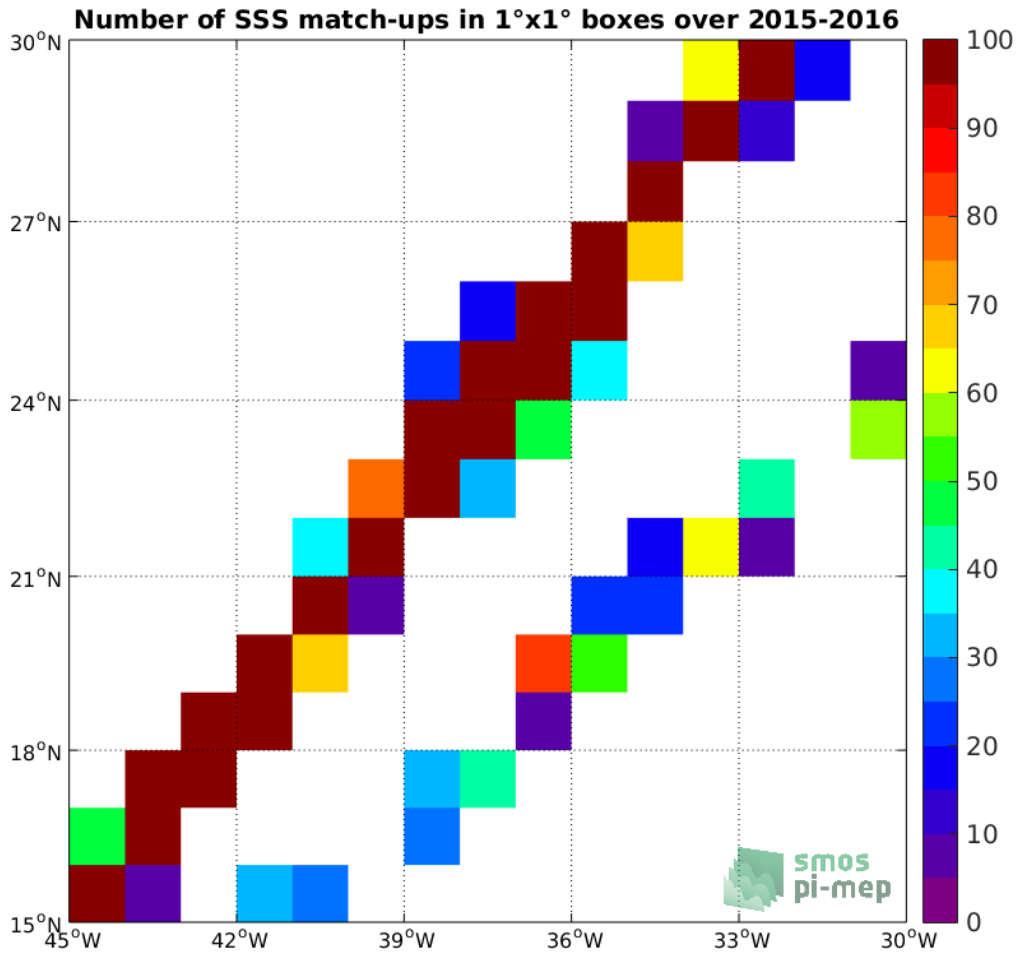
Figure 4: Number of SSS match-ups between TSG-LEGOS-DM SSS and the SMAP-L2-RSS-V3-70KM SSS product for the SPURS 1 Pi-MEP region over 1°x1° boxes and for the full satellite product period.
