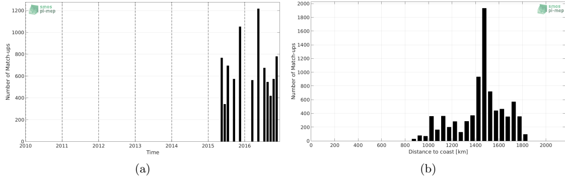
Figure 1: Number of match-ups between TSG-LEGOS-DM and SMAP-L2-RSS-V3-70KM SSS as a function of time (a) and as function of the distance to coast (b) over the SPURS 1 Pi-MEP region and for the full satellite product period.
