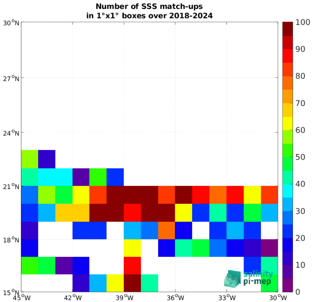
Figure 5: Number of SSS match-ups between TSG (SAMOS) SSS and the SMAP SSS L2 v5.0 (JPL) SSS product for the SPURS 1 Pi-MEP region over 1°x1° boxes and for the full satellite product period.
