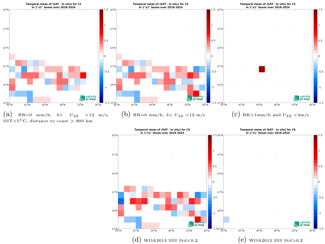
Figure 14: Temporal mean gridded over spatial boxes of size 1^\circ \times 1^\circ of \Delta\text{SSS} (SMAP SSS L2 v5.0 (JPL) - TSG (SAMOS)) for 5 different subdatasets corresponding to: \text{RR}=0 mm/h, 3 < U_{10} < 12 m/s, \text{SST} > 5^\circ\text{C} , distance to coast > 800 km (a), \text{RR}=0 mm/h, 3 < U_{10} < 12 m/s (b), \text{RR} > 1\text{mm/h} and U_{10} < 4\text{m/s} (c), WOA2013 SSS Std < 0.2 (d), WOA2013 SSS Std > 0.2 (e).
