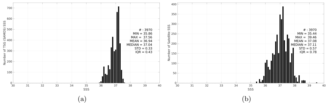
Figure 3: Histograms of SSS from TSG (SAMOS) (a) and SMAP SSS L2 v5.0 (JPL) (b) considering all match-up pairs per bins of 0.1 over the SPURS 1 Pi-MEP region and for the full satellite product period.
