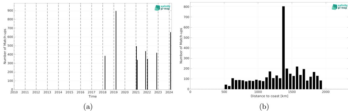
Figure 2: Number of match-ups between TSG (SAMOS) and SMAP SSS L2 v5.0 (JPL) SSS as a function of time (a) and as function of the distance to coast (b) over the SPURS 1 Pi-MEP region and for the full satellite product period.
