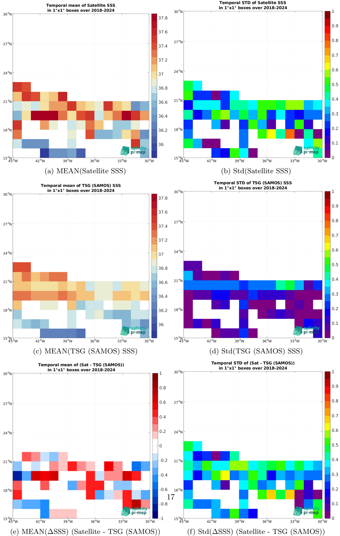
Figure 7: Temporal mean (left) and Std (right) of SSS from SMAP SSS L2 v5.0 (JPL) (top), TSG (SAMOS) (middle), and of \Delta SSS (Satellite - TSG (SAMOS)). Only match-up pairs are used to generate these maps.
