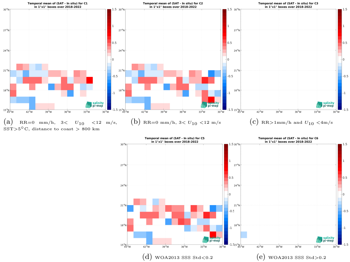
Figure 12: Temporal mean gridded over spatial boxes of size 1^\circ \times 1^\circ of \Delta\text{SSS} (SMAP SSS L2 v5.0 (JPL) - TSG (SAMOS)) for 5 different subdatasets corresponding to: \text{RR}=0 mm/h, 3 < U_{10} < 12 m/s, \text{SST} > 5^\circ\text{C} , distance to coast > 800 km (a), \text{RR}=0 mm/h, 3 < U_{10} < 12 m/s (b), \text{RR} > 1\text{mm/h} and U_{10} < 4\text{m/s} (c), WOA2013 SSS Std < 0.2 (d), WOA2013 SSS Std > 0.2 (e).
