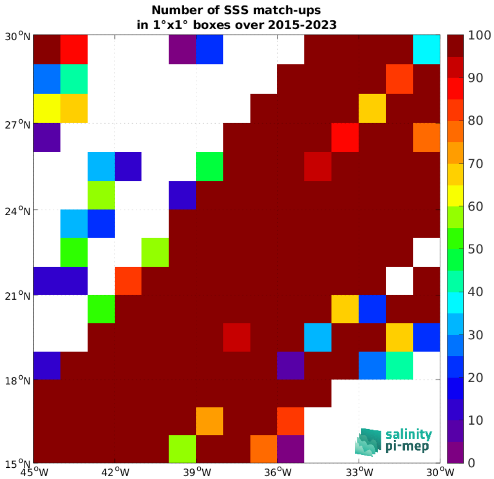
Figure 5: Number of SSS match-ups between TSG (LEGOS-DM) SSS and the SMAP SSS L2 v5.0 (JPL) SSS product for the SPURS 1 Pi-MEP region over 1°×1° boxes and for the full satellite product period.
