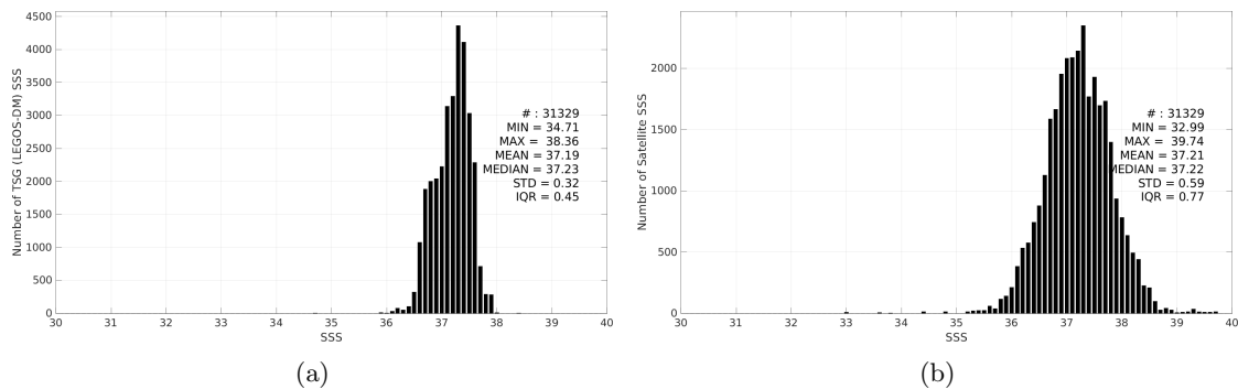
Figure 3: Histograms of SSS from TSG (LEGOS-DM) (a) and SMAP SSS L2 v5.0 (JPL) (b) considering all match-up pairs per bins of 0.1 over the SPURS 1 Pi-MEP region and for the full satellite product period.
