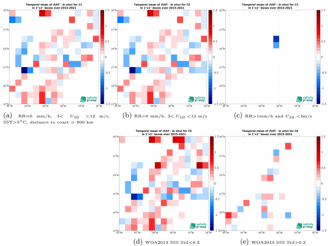
Figure 14: Temporal mean gridded over spatial boxes of size 1^\circ \times 1^\circ of \Delta\text{SSS} (SMAP SSS L2 v5.0 (JPL) - TSG (LEGOS-DM)) for 5 different subdatasets corresponding to:RR=0 mm/h, 3 < U_{10} < 12 m/s, SST>5°C, distance to coast > 800 km (a), RR=0 mm/h, 3 < U_{10} < 12 m/s (b), RR>1mm/h and U_{10} < 4 m/s (c), WOA2013 SSS Std<0.2 (d), WOA2013 SSS Std>0.2 (e).
