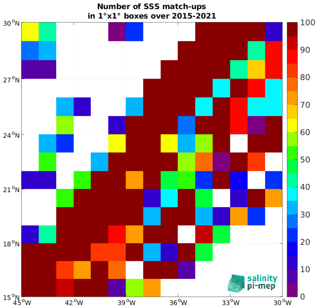
Figure 5: Number of SSS match-ups between TSG (LEGOS-DM) SSS and the SMAP SSS L2 v5.0 (JPL) SSS product for the SPURS 1 Pi-MEP region over 1^\circ \times 1^\circ boxes and for the full satellite product period.
