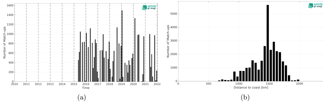
Figure 2: Number of match-ups between TSG (LEGOS-DM) and SMAP SSS L2 v5.0 (JPL) SSS as a function of time (a) and as function of the distance to coast (b) over the SPURS 1 Pi-MEP region and for the full satellite product period.
