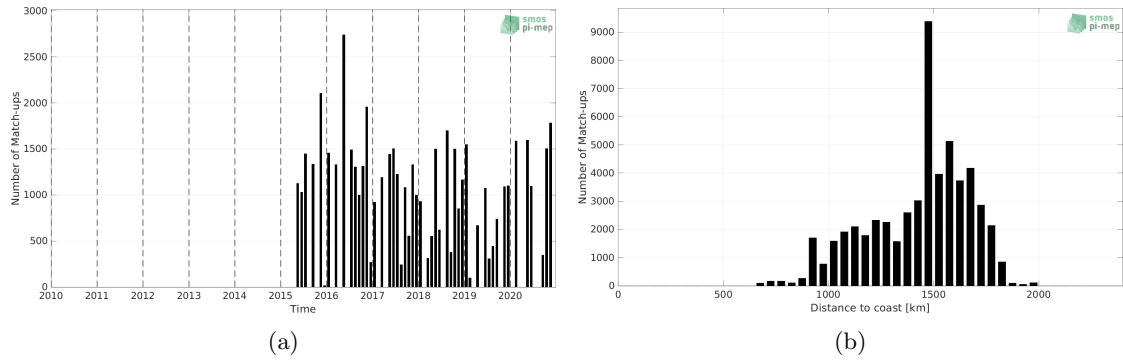
Figure 1: Number of match-ups between TSG (LEGOS-DM) and SMAP SSS L2 v5.0 (JPL) SSS as a function of time (a) and as function of the distance to coast (b) over the SPURS 1 Pi-MEP region and for the full satellite product period.
