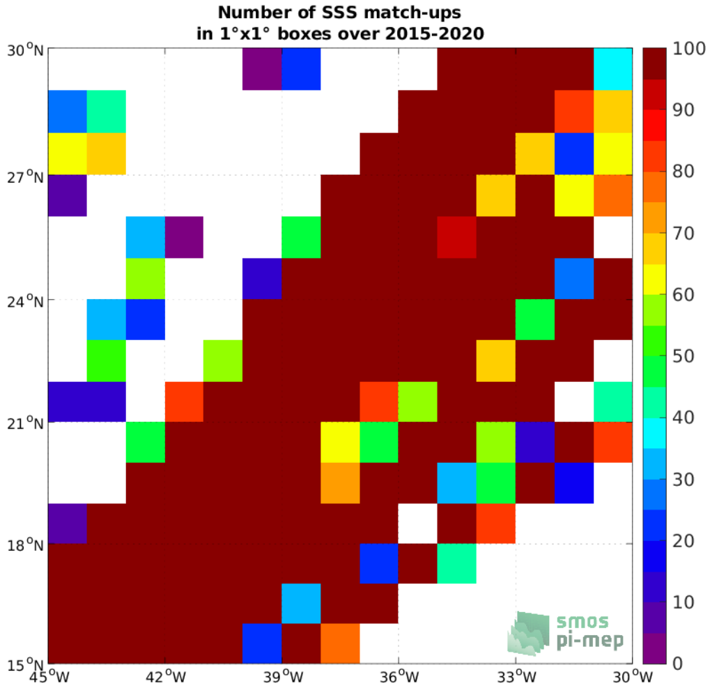
Figure 4: Number of SSS match-ups between TSG (LEGOS-DM) SSS and the SMAP SSS L2 v5.0 (JPL) SSS product for the SPURS 1 Pi-MEP region over 1^\circ \times 1^\circ boxes and for the full satellite product period.
