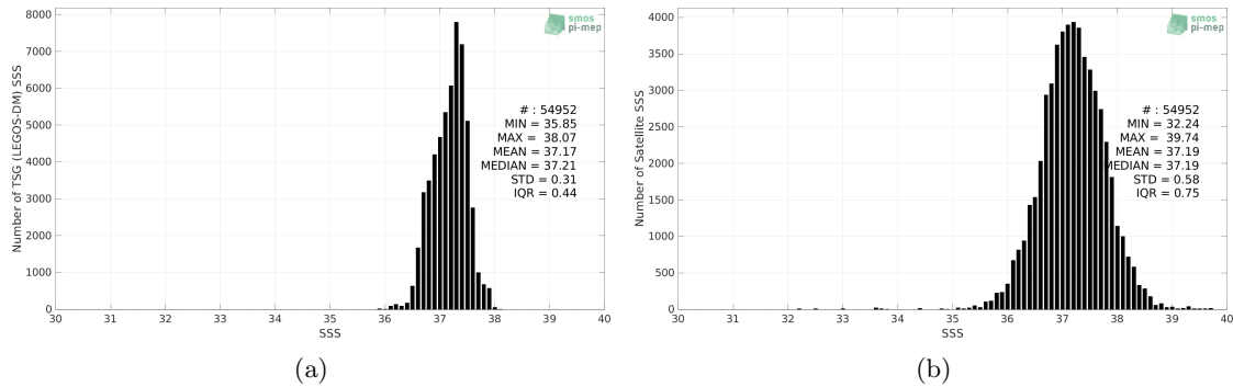
Figure 2: Histograms of SSS from TSG (LEGOS-DM) (a) and SMAP SSS L2 v5.0 (JPL) (b) considering all match-up pairs per bins of 0.1 over the SPURS 1 Pi-MEP region and for the full satellite product period.
