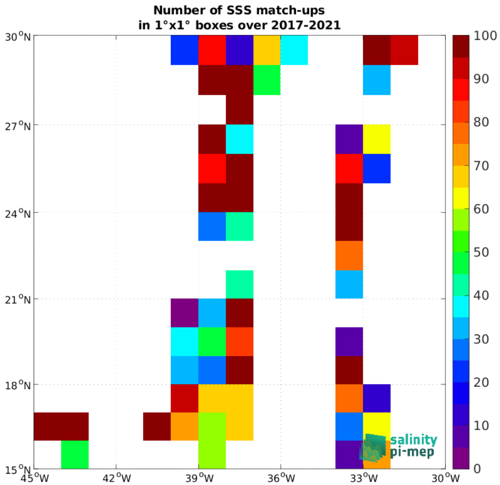
Figure 5: Number of SSS match-ups between TSG (GOSUD-Sailing-ship) SSS and the SMAP SSS L2 v5.0 (JPL) SSS product for the SPURS 1 Pi-MEP region over 1^\circ \times 1^\circ boxes and for the full satellite product period.
