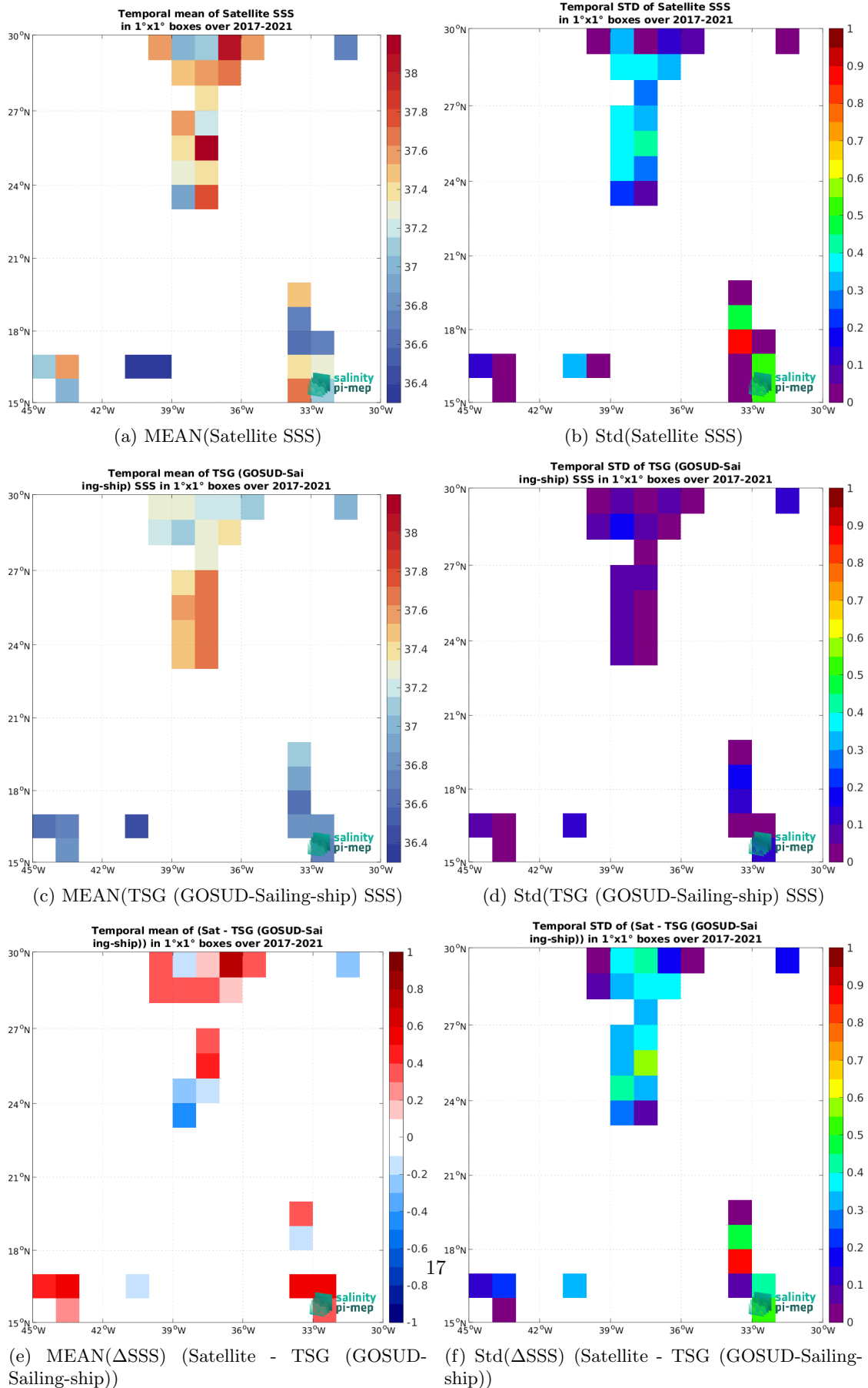
Figure 7: Temporal mean (left) and Std (right) of SSS from SMAP SSS L2 v5.0 (JPL) (top), TSG (GOSUD-Sailing-ship) (middle), and of \Delta SSS (Satellite - TSG (GOSUD-Sailing-ship)). Only match-up pairs are used to generate these maps.
