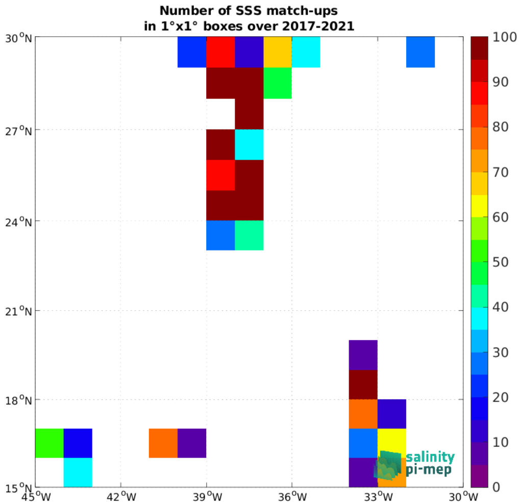
Figure 5: Number of SSS match-ups between TSG (GOSUD-Sailing-ship) SSS and the SMAP SSS L2 v5.0 (JPL) SSS product for the SPURS 1 Pi-MEP region over 1°×1° boxes and for the full satellite product period.
