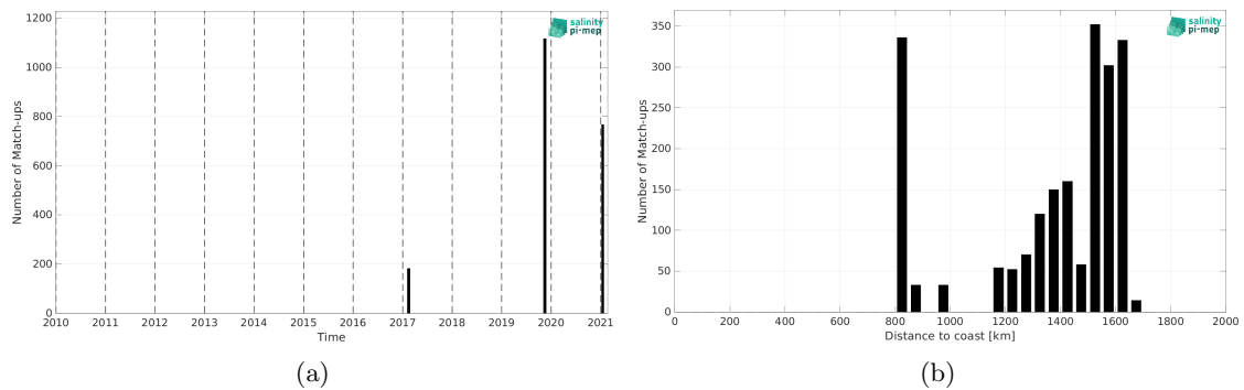
Figure 2: Number of match-ups between TSG (GOSUD-Sailing-ship) and SMAP SSS L2 v5.0 (JPL) SSS as a function of time (a) and as function of the distance to coast (b) over the SPURS 1 Pi-MEP region and for the full satellite product period.
