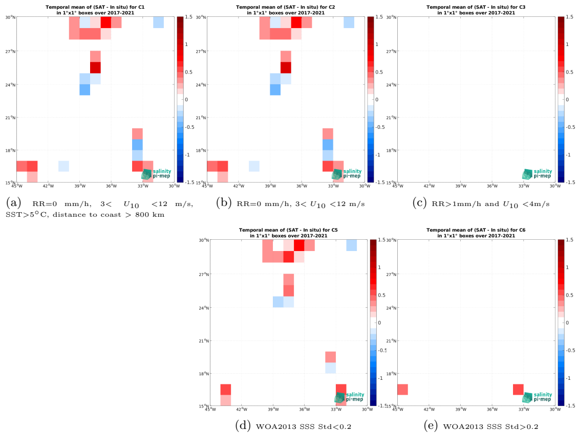
Figure 14: Temporal mean gridded over spatial boxes of size 1^\circ \times 1^\circ of \Delta\text{SSS} (SMAP SSS L2 v5.0 (JPL) - TSG (GOSUD-Sailing-ship)) for 5 different subdatasets corresponding to: \text{RR}=0 \text{ mm/h} , 3 < U_{10} < 12 \text{ m/s} , \text{SST} > 5^\circ\text{C} , distance to coast > 800 \text{ km} (a), \text{RR}=0 \text{ mm/h} , 3 < U_{10} < 12 \text{ m/s} (b), \text{RR} > 1\text{mm/h} and U_{10} < 4\text{m/s} (c), WOA2013 SSS Std < 0.2 (d), WOA2013 SSS Std > 0.2 (e).
