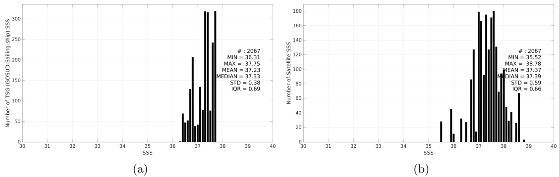
Figure 3: Histograms of SSS from TSG (GOSUD-Sailing-ship) (a) and SMAP SSS L2 v5.0 (JPL) (b) considering all match-up pairs per bins of 0.1 over the SPURS 1 Pi-MEP region and for the full satellite product period.
