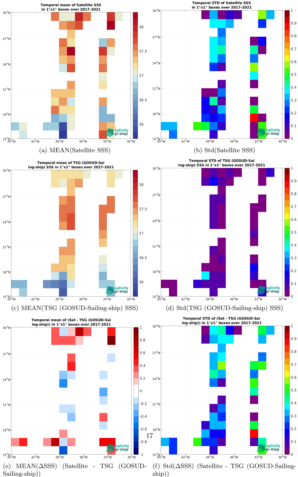
Figure 6: Temporal mean (left) and Std (right) of SSS from SMAP SSS L2 v5.0 (JPL) (top), TSG (GOSUD-Sailing-ship) (middle), and of \Delta SSS (Satellite - TSG (GOSUD-Sailing-ship)). Only match-up pairs are used to generate these maps.
