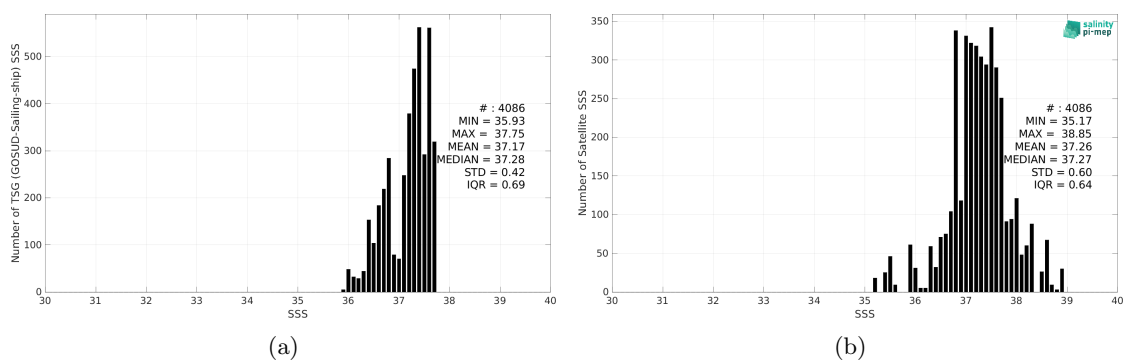
Figure 2: Histograms of SSS from TSG (GOSUD-Sailing-ship) (a) and SMAP SSS L2 v5.0 (JPL) (b) considering all match-up pairs per bins of 0.1 over the SPURS 1 Pi-MEP region and for the full satellite product period.
