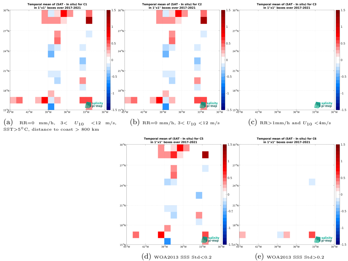
Figure 12: Temporal mean gridded over spatial boxes of size 1^\circ \times 1^\circ of \Delta\text{SSS} (SMAP SSS L2 v5.0 (JPL) - TSG (GOSUD-Sailing-ship)) for 5 different subdatasets corresponding to:RR=0 mm/h, 3 < U_{10} < 12 m/s, SST >5^\circ\text{C} , distance to coast > 800 km (a), RR=0 mm/h, 3 < U_{10} < 12 m/s (b), RR >1 mm/h and U_{10} < 4 m/s (c), WOA2013 SSS Std <0.2 (d), WOA2013 SSS Std >0.2 (e).
