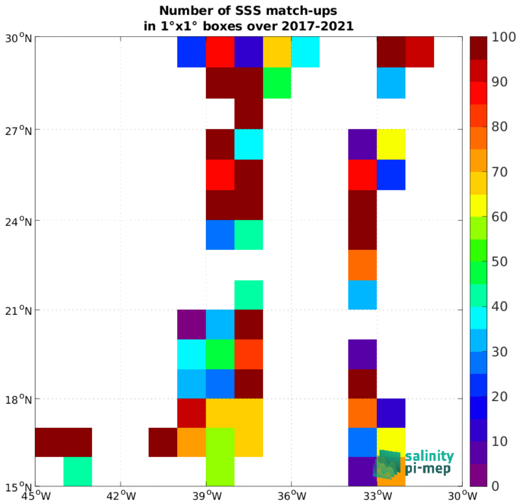
Figure 4: Number of SSS match-ups between TSG (GOSUD-Sailing-ship) SSS and the SMAP SSS L2 v5.0 (JPL) SSS product for the SPURS 1 Pi-MEP region over 1^\circ \times 1^\circ boxes and for the full satellite product period.
