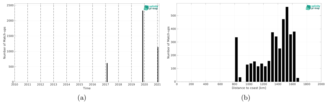
Figure 1: Number of match-ups between TSG (GOSUD-Sailing-ship) and SMAP SSS L2 v5.0 (JPL) SSS as a function of time (a) and as function of the distance to coast (b) over the SPURS 1 Pi-MEP region and for the full satellite product period.
