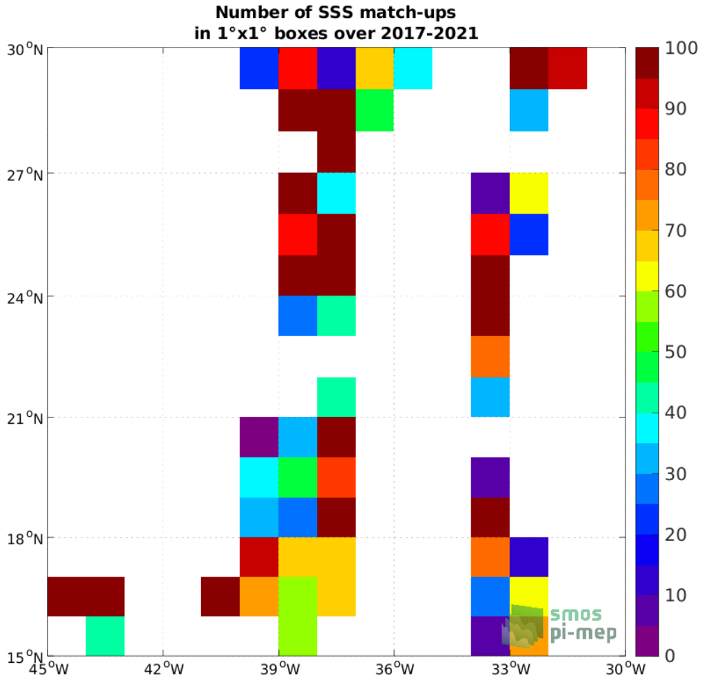
Figure 4: Number of SSS match-ups between TSG (GOSUD-Sailing-ship) SSS and the SMAP SSS L2 v5.0 (JPL) SSS product for the SPURS 1 Pi-MEP region over 1°x1° boxes and for the full satellite product period.
