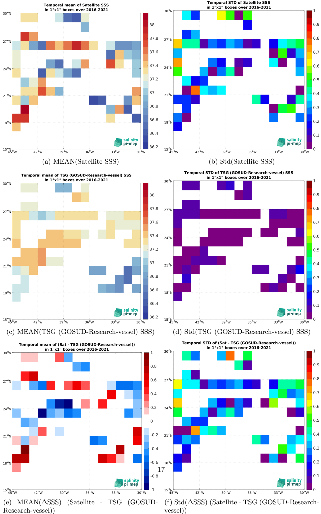
Figure 7: Temporal mean (left) and Std (right) of SSS from SMAP SSS L2 v5.0 (JPL) (top), TSG (GOSUD-Research-vessel) (middle), and of \Delta SSS (Satellite - TSG (GOSUD-Research-vessel)). Only match-up pairs are used to generate these maps.
