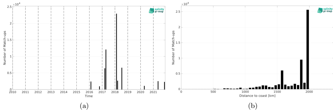
Figure 1: Number of match-ups between TSG (GOSUD-Research-vessel) and SMAP SSS L2 v5.0 (JPL) SSS as a function of time (a) and as function of the distance to coast (b) over the SPURS 1 Pi-MEP region and for the full satellite product period.
