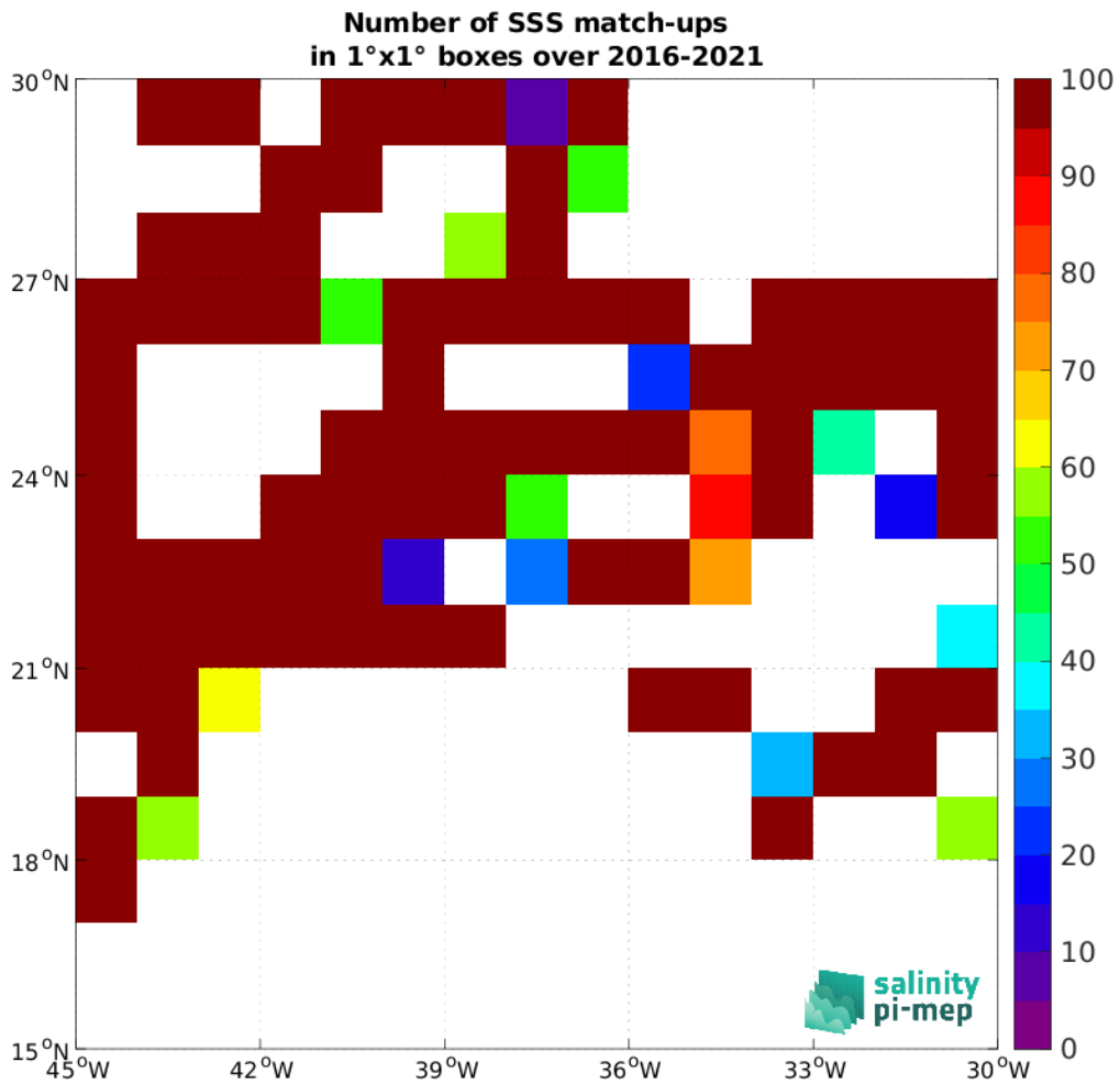
Figure 4: Number of SSS match-ups between TSG (GOSUD-Research-vessel) SSS and the SMAP SSS L2 v5.0 (JPL) SSS product for the SPURS 1 Pi-MEP region over 1°x1° boxes and for the full satellite product period.
