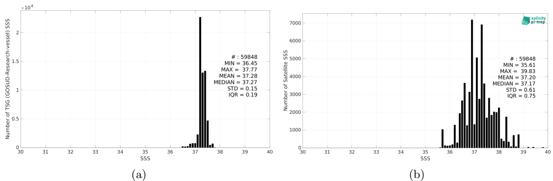
Figure 2: Histograms of SSS from TSG (GOSUD-Research-vessel) (a) and SMAP SSS L2 v5.0 (JPL) (b) considering all match-up pairs per bins of 0.1 over the SPURS 1 Pi-MEP region and for the full satellite product period.
