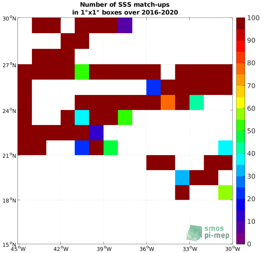
Figure 4: Number of SSS match-ups between TSG (GOSUD-Research-vessel) SSS and the SMAP SSS L2 v5.0 (JPL) SSS product for the SPURS 1 Pi-MEP region over 1^\circ \times 1^\circ boxes and for the full satellite product period.
