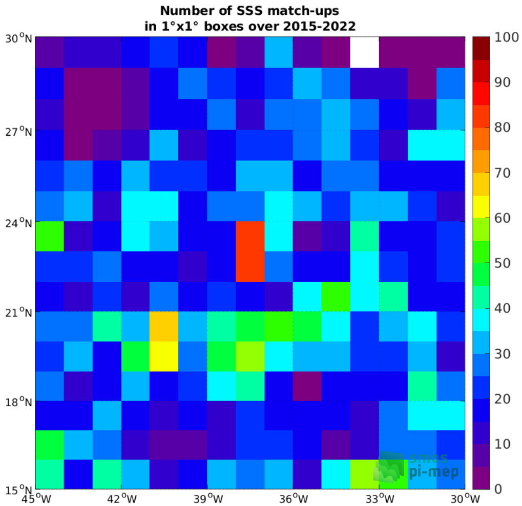
Figure 4: Number of SSS match-ups between Argo SSS and the SMAP SSS L2 v5.0 (JPL) SSS product for the SPURS 1 Pi-MEP region over 1°×1° boxes and for the full satellite product period.
