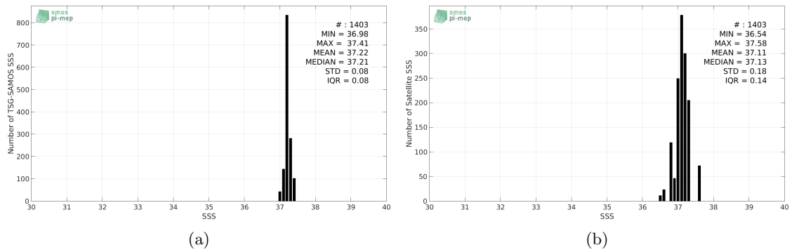
Figure 2: Histograms of SSS from TSG-SAMOS (a) and SMAP-L2-JPL-V4 (b) considering all match-up pairs per bins of 0.1 over the SPURS 1 Pi-MEP region and for the full satellite product period.
