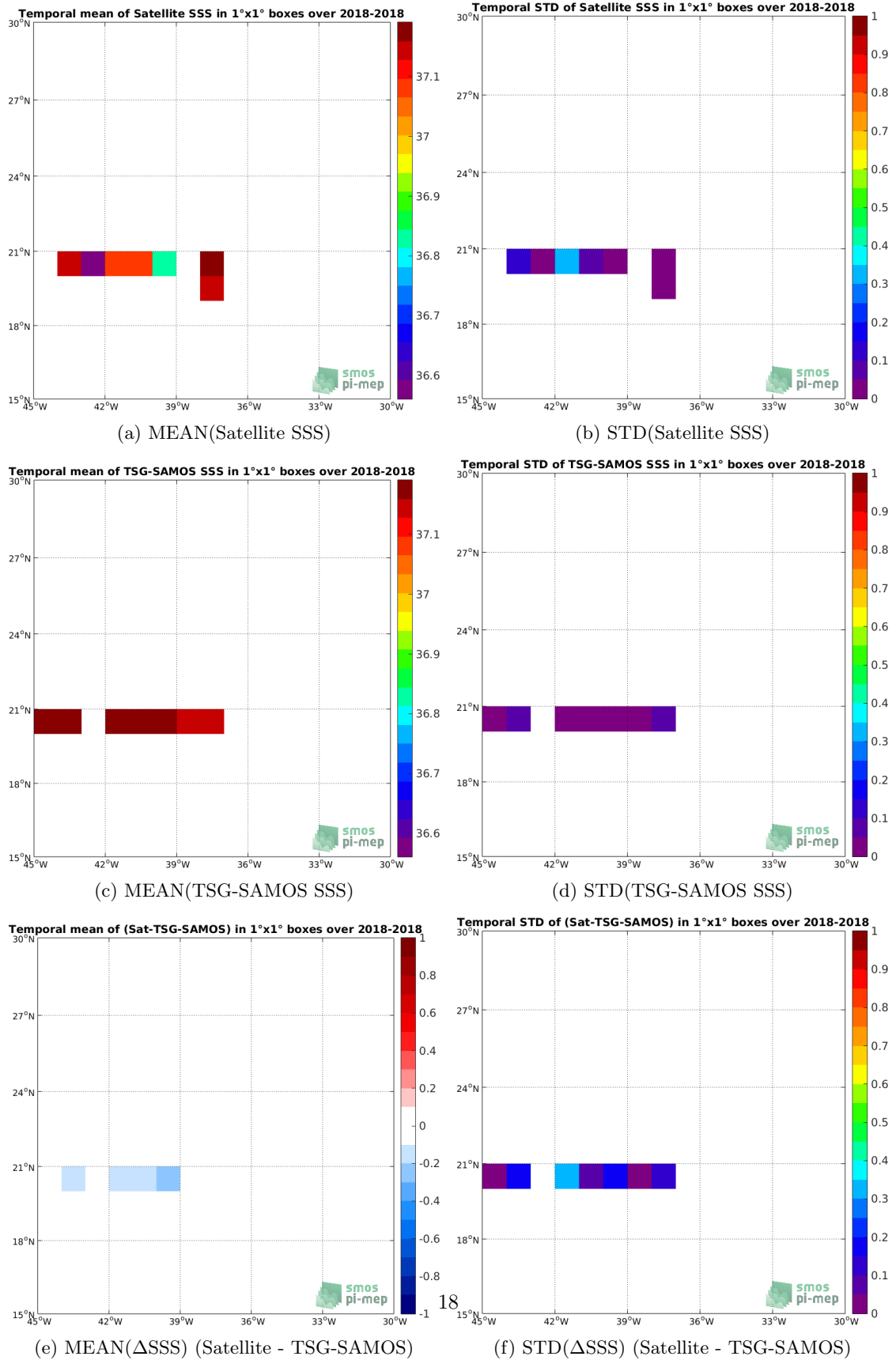
Figure 6: Temporal mean (left) and STD (right) of SSS from SMAP-L2-JPL-V4 (top), TSG-SAMOS (middle), and of \Delta SSS (Satellite - TSG-SAMOS). Only match-up pairs are used to generate these maps.
