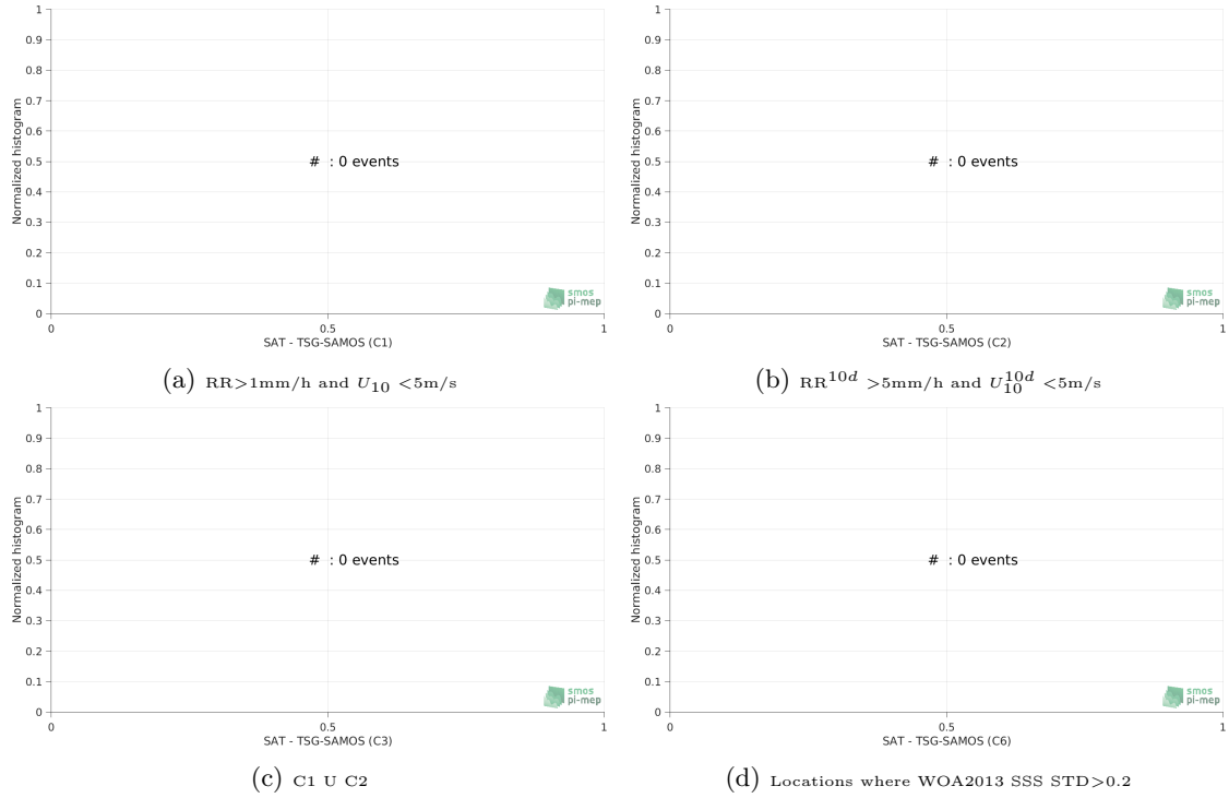
Figure 13: Normalized histogram of \Delta\text{SSS} (SMAP-L2-JPL-V4 - TSG-SAMOS) for 6 different subdatasets corresponding to: \text{RR} > 1\text{mm/h} and U_{10} < 5\text{m/s} (a), \text{RR}^{10d} > 5\text{mm/h} and U_{10}^{10d} < 5\text{m/s} (b), C1 U C2 (c), Locations where WOA2013 SSS STD > 0.2 (d).
