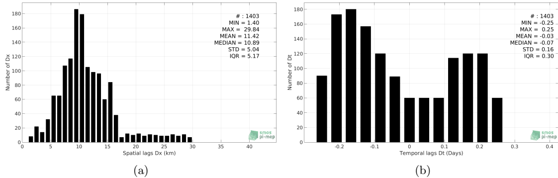
Figure 5: Histograms of the spatial (a) and temporal (b) lags between the time of the TSG-SAMOS measurements and the date of the corresponding SMAP-L2-JPL-V4 SSS product.
