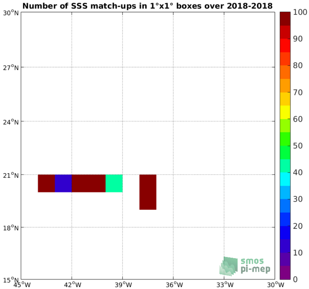
Figure 4: Number of SSS match-ups between TSG-SAMOS SSS and the SMAP-L2-JPL-V4 SSS product for the SPURS 1 Pi-MEP region over 1°x1° boxes and for the full satellite product period.
