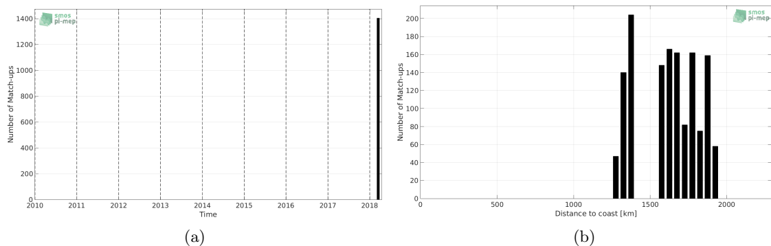
Figure 1: Number of match-ups between TSG-SAMOS and SMAP-L2-JPL-V4 SSS as a function of time (a) and as function of the distance to coast (b) over the SPURS 1 Pi-MEP region and for the full satellite product period.
