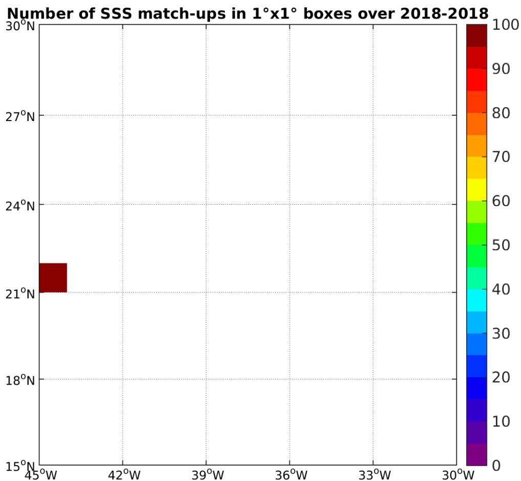
Figure 4: Number of SSS match-ups between TSG-SAMOS SSS and the SMAP-L2-JPL-V4 SSS product for the SPURS 1 Pi-MEP region over 1°x1° boxes and for the full satellite product period.
