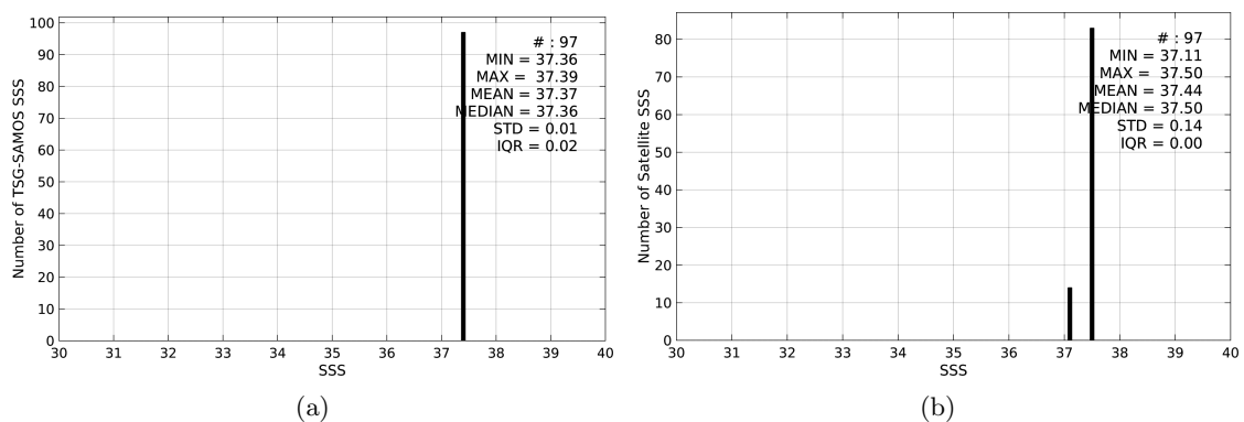
Figure 2: Histograms of SSS from TSG-SAMOS (a) and SMAP-L2-JPL-V4 (b) considering all match-up pairs per bins of 0.1 over the SPURS 1 Pi-MEP region and for the full satellite product period.
