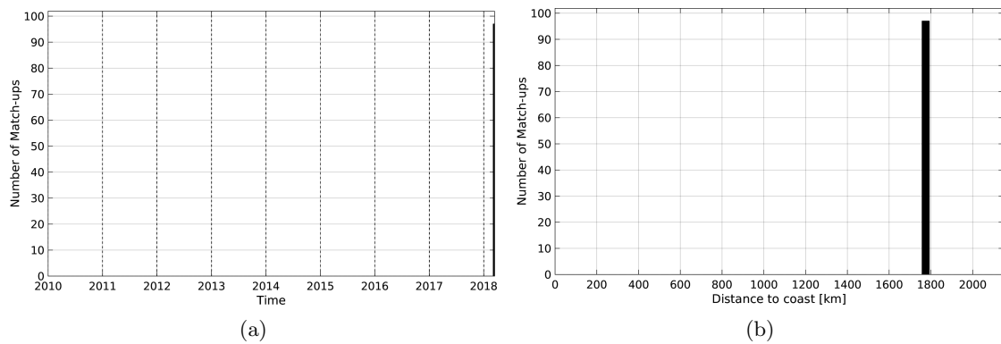
Figure 1: Number of match-ups between TSG-SAMOS and SMAP-L2-JPL-V4 SSS as a function of time (a) and as function of the distance to coast (b) over the SPURS 1 Pi-MEP region and for the full satellite product period.
