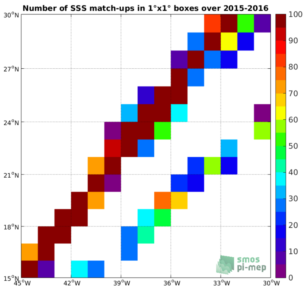
Figure 4: Number of SSS match-ups between TSG-LEGOS-DM SSS and the SMAP-L2-JPL-V4 SSS product for the SPURS 1 Pi-MEP region over 1°x1° boxes and for the full satellite product period.
