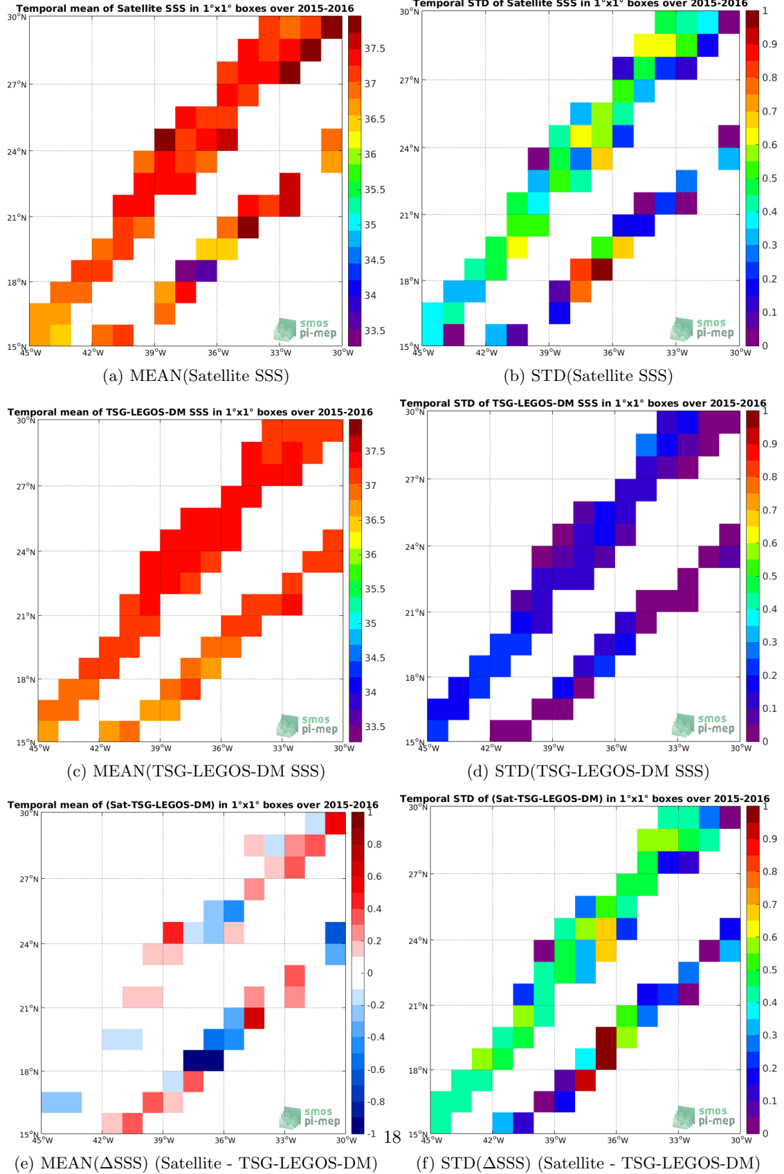
Figure 6: Temporal mean (left) and STD (right) of SSS from SMAP-L2-JPL-V4 (top), TSG-LEGOS-DM (middle), and of \Delta SSS (Satellite - TSG-LEGOS-DM). Only match-up pairs are used to generate these maps.
