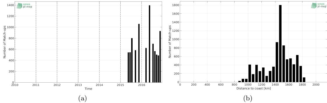
Figure 1: Number of match-ups between TSG-LEGOS-DM and SMAP-L2-JPL-V4 SSS as a function of time (a) and as function of the distance to coast (b) over the SPURS 1 Pi-MEP region and for the full satellite product period.
