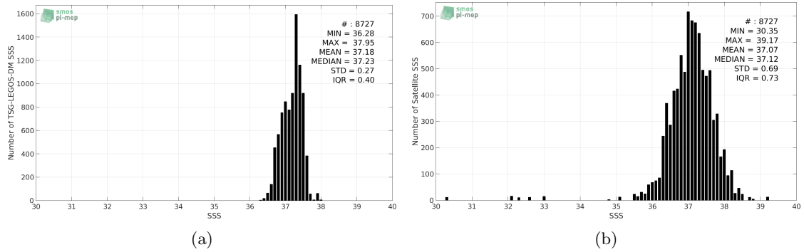
Figure 2: Histograms of SSS from TSG-LEGOS-DM (a) and SMAP-L2-JPL-V4 (b) considering all match-up pairs per bins of 0.1 over the SPURS 1 Pi-MEP region and for the full satellite product period.
